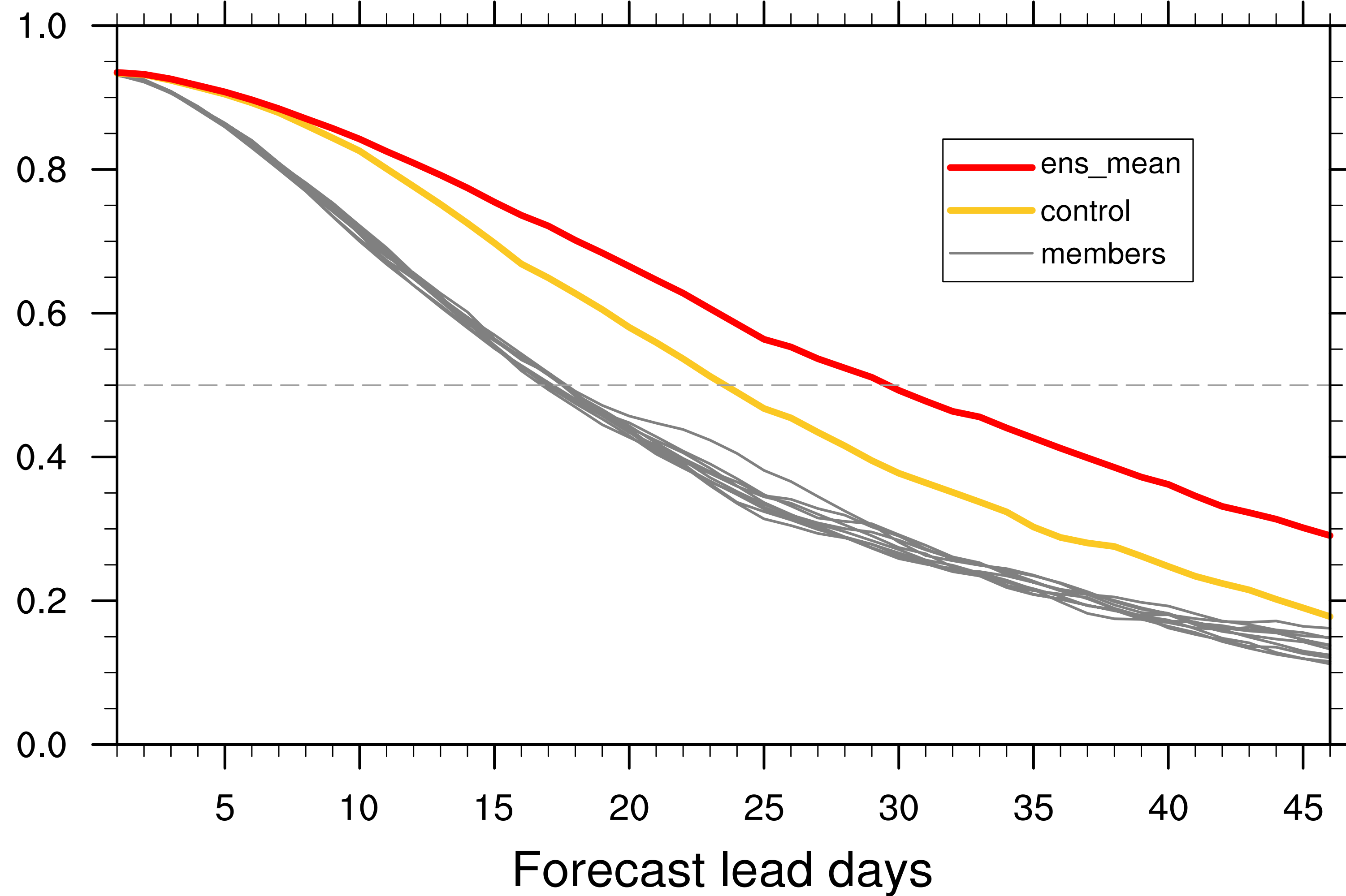
(a) ECMWF
