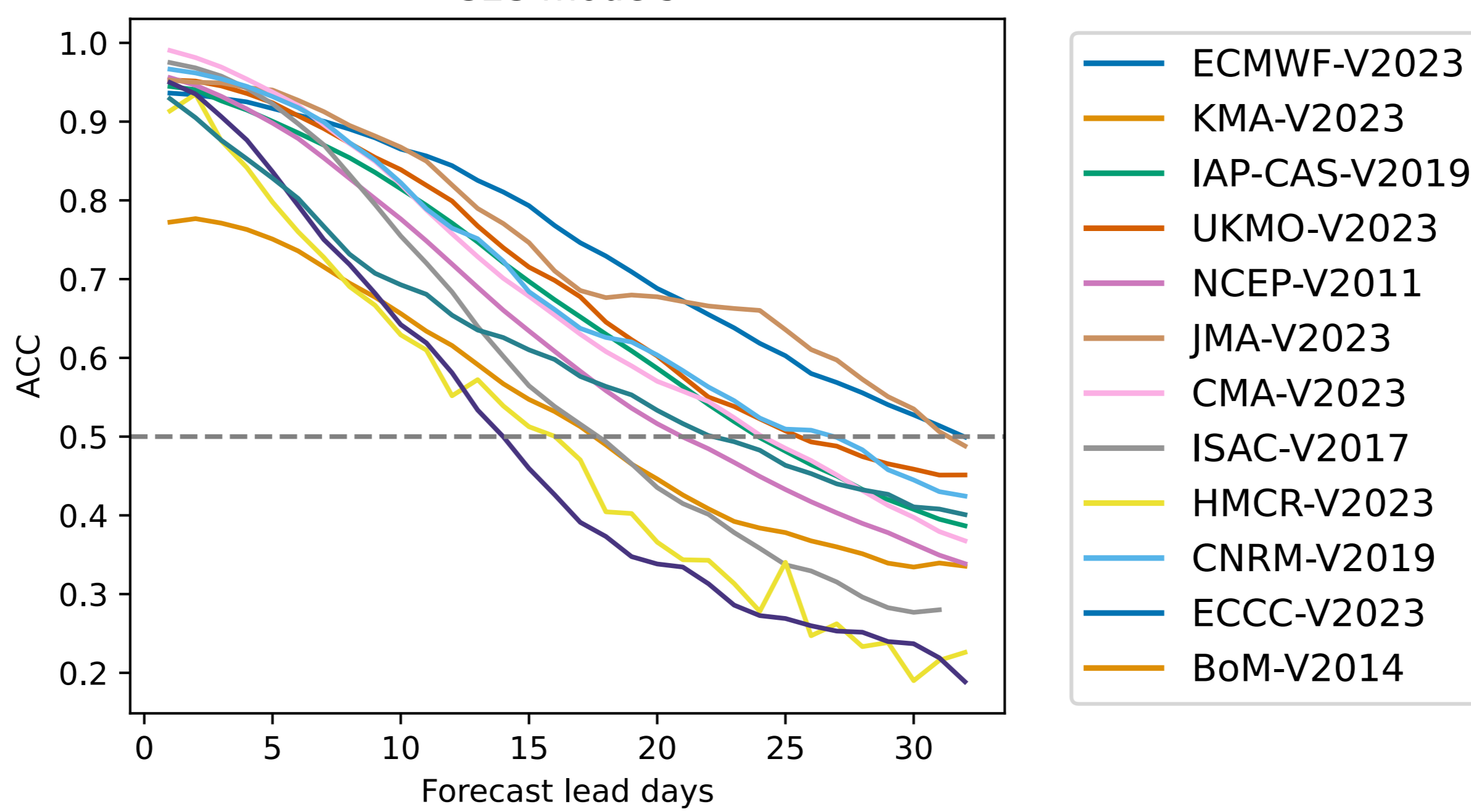
S2S models
