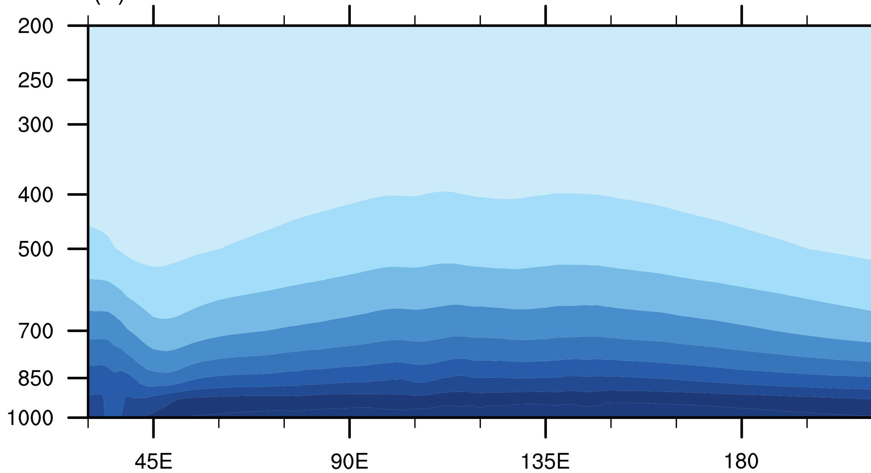
(a) Obs
