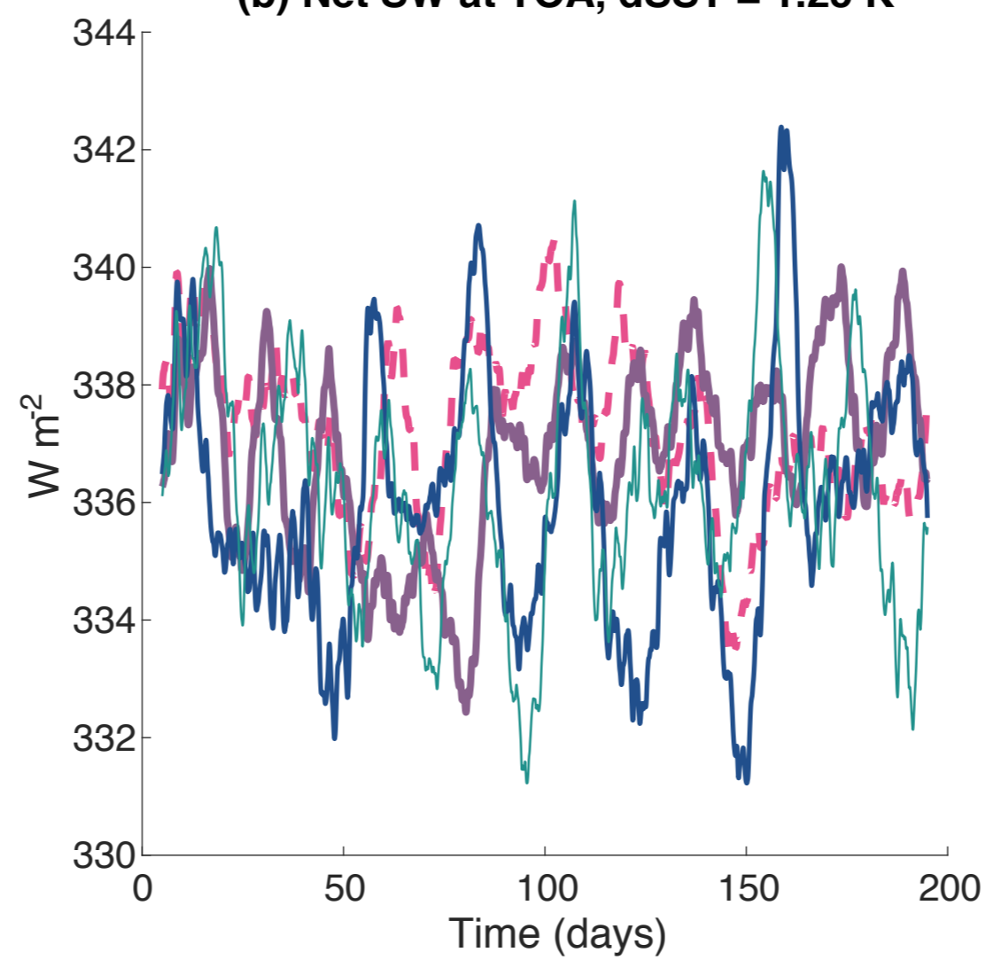
(b) Net SW at TOA, dSST = 1.25 K
