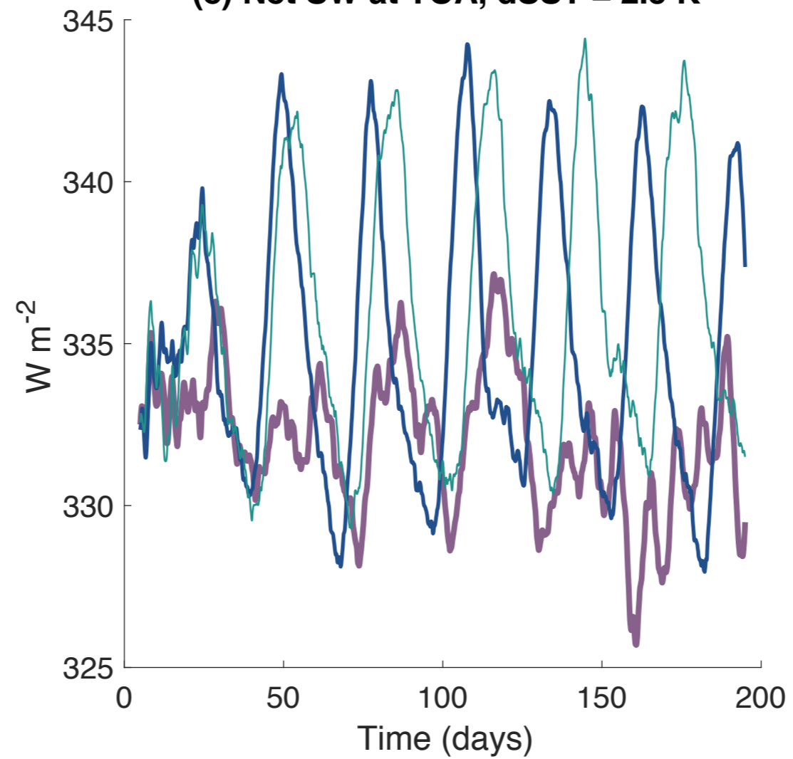
(e) Net SW at TOA, dSST = 2.5 K
