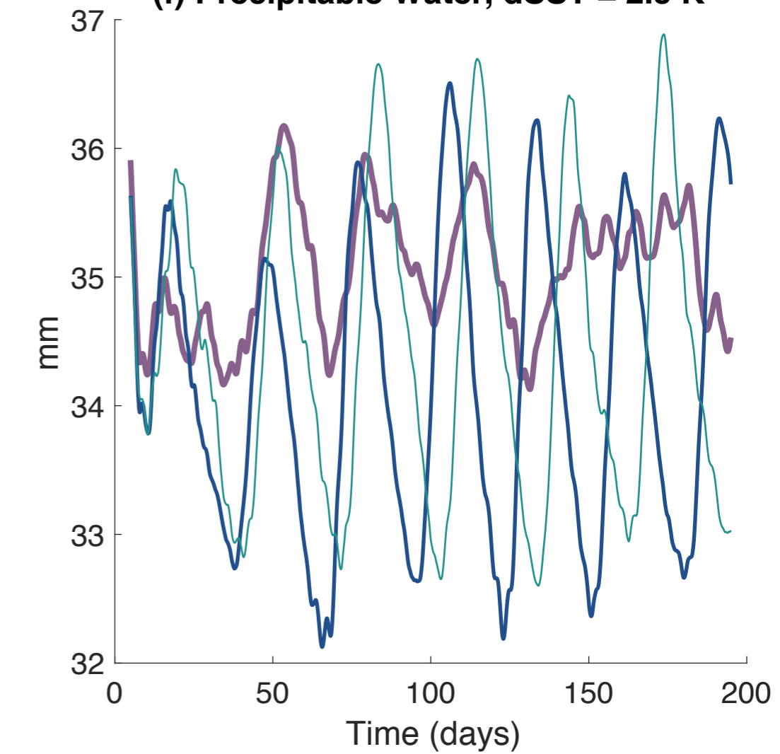
(f) Precipitable Water, dSST = 2.5 K
