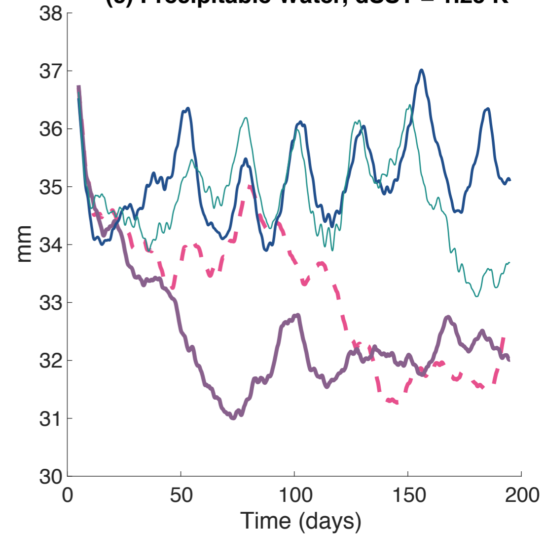
(c) Precipitable Water, dSST = 1.25 K
