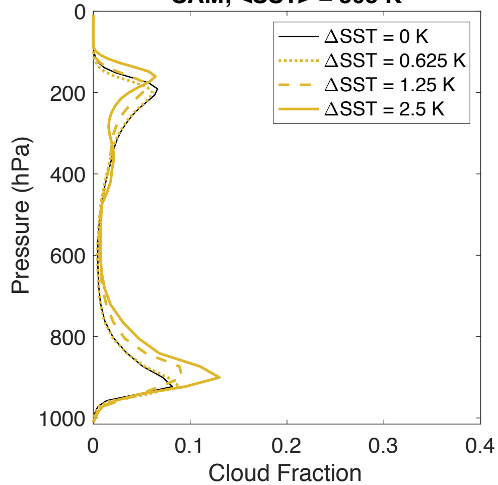
SAM; <SST> = 305 K
