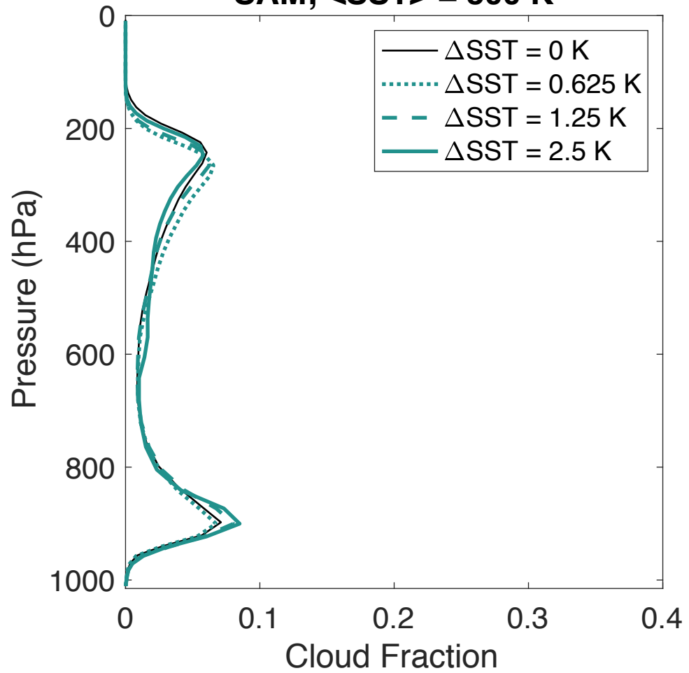
SAM; <SST> = 300 K
