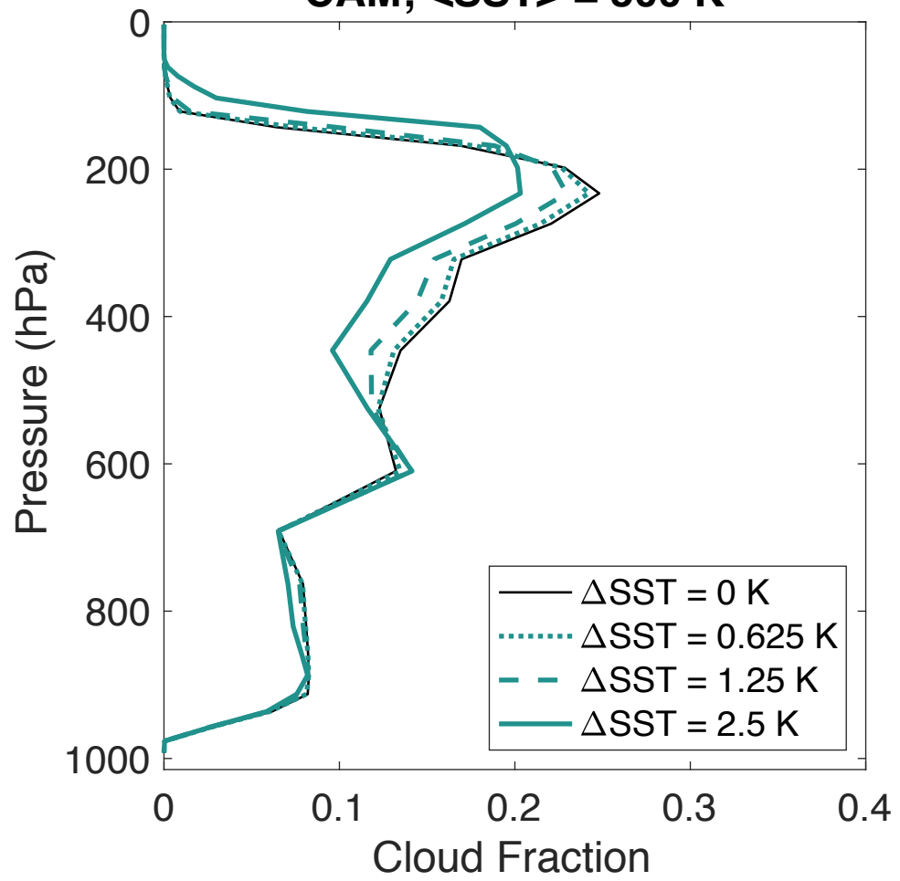
CAM; <SST> = 300 K
