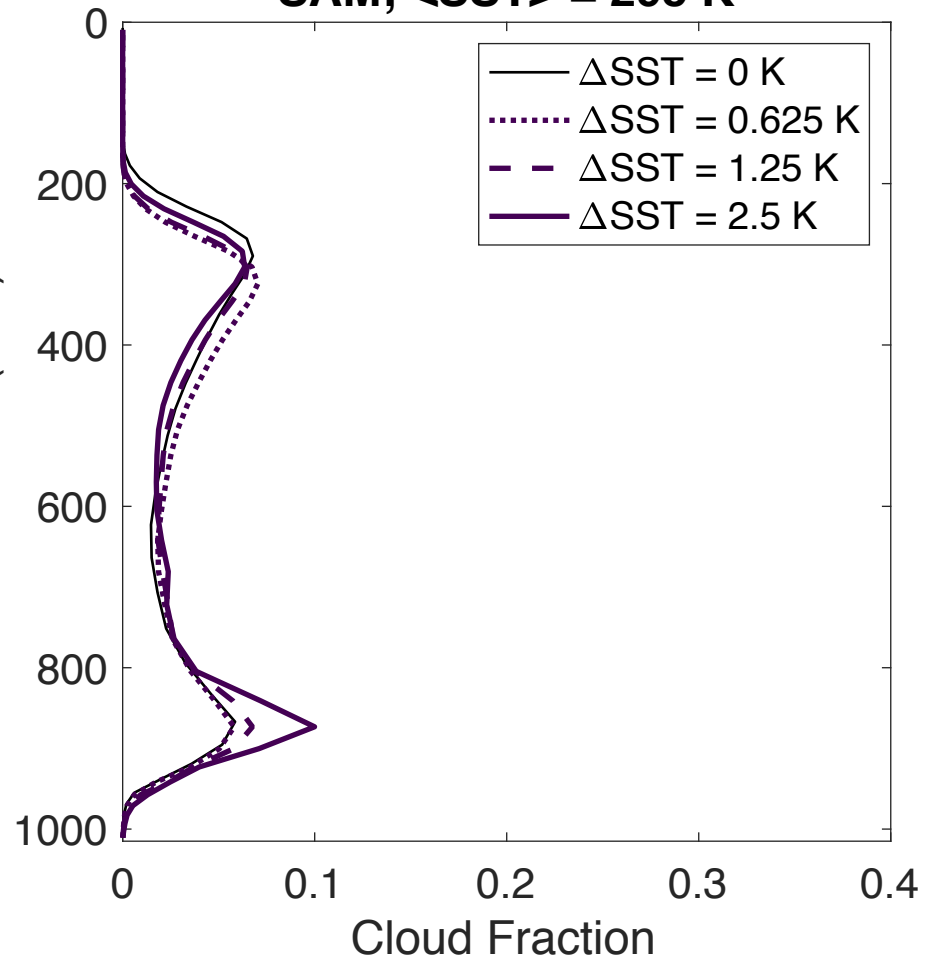
SAM; <SST> = 295 K
