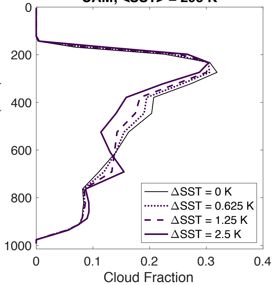
CAM; <SST> = 295 K
