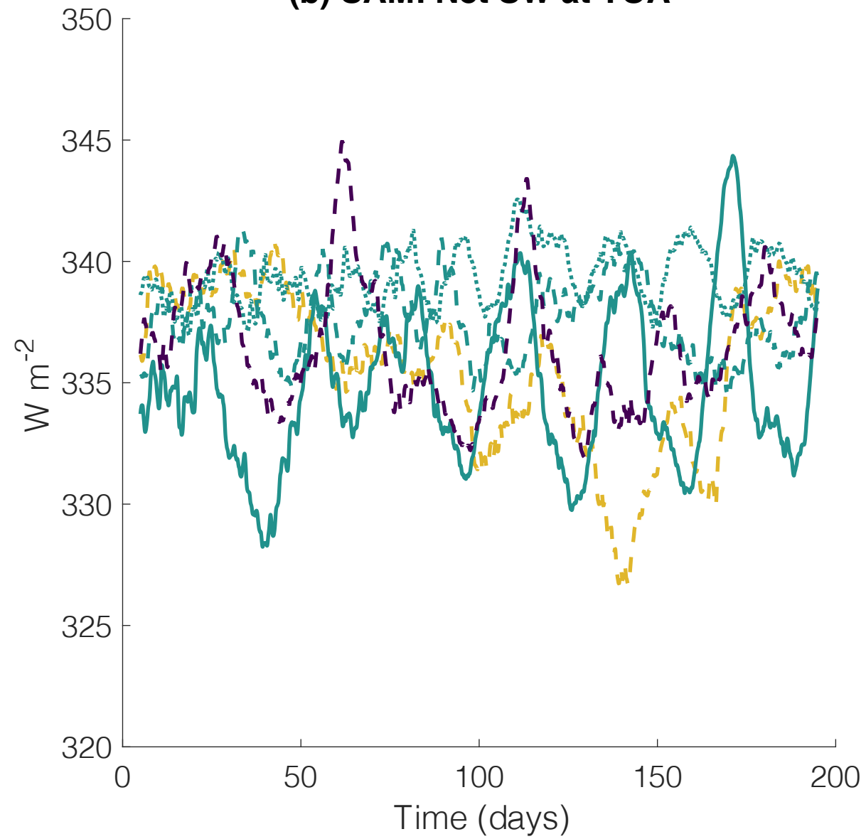
(b) SAM: Net SW at TOA
