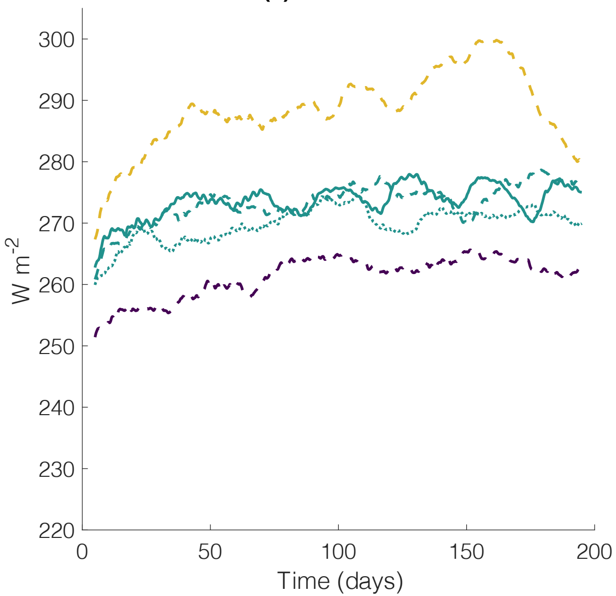
(a) SAM: OLR
