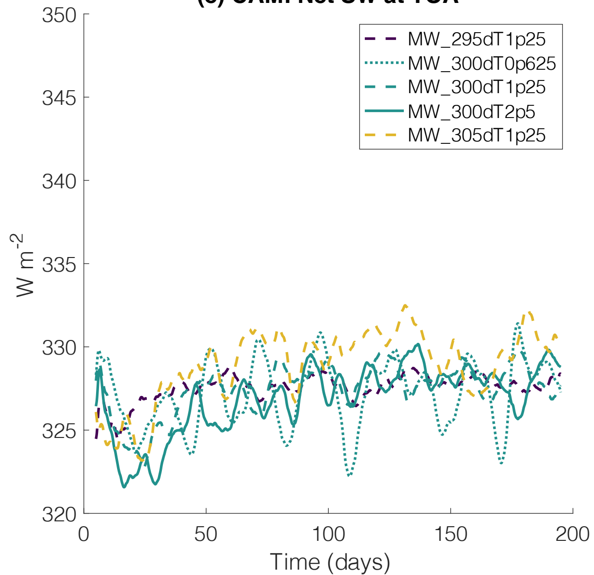
(e) CAM: Net SW at TOA
