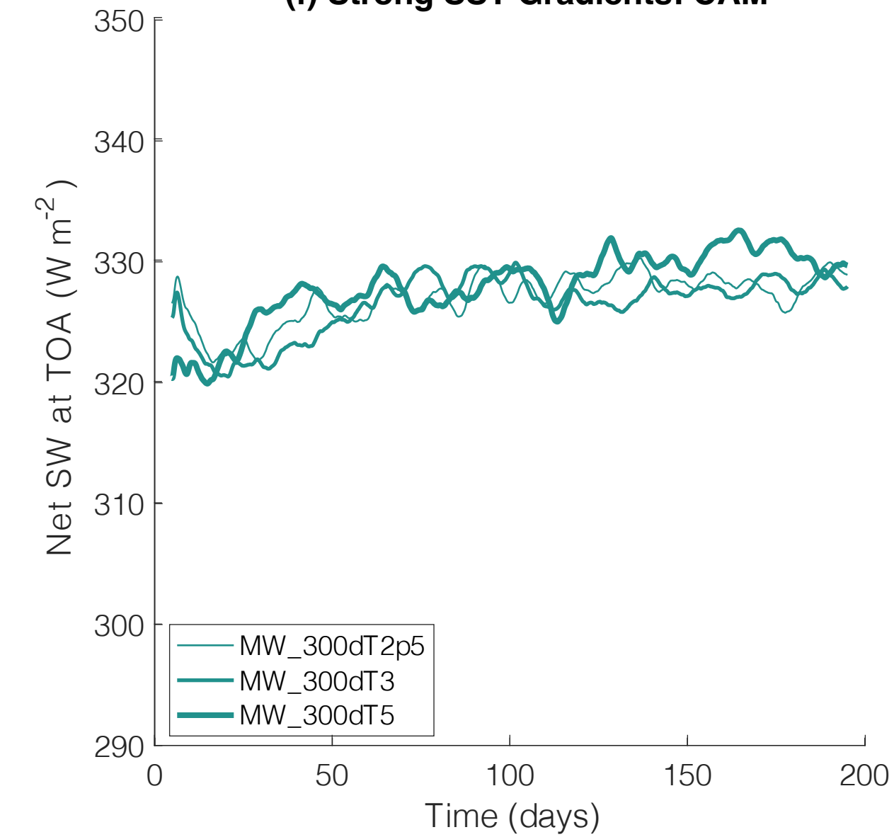
(f) Strong SST Gradients: CAM
