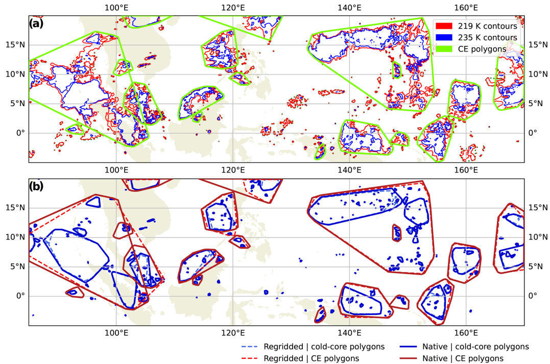
Figure 3. CEs identified on 8 September 2006 at 22:00 UTC (10 h in) for the sample MPAS datasets. (a) Contours of the native MPAS output and associated CE polygons. (b) CEs derived from native (solid lines) MPAS output and regridded (dashed lines) MPAS output.
