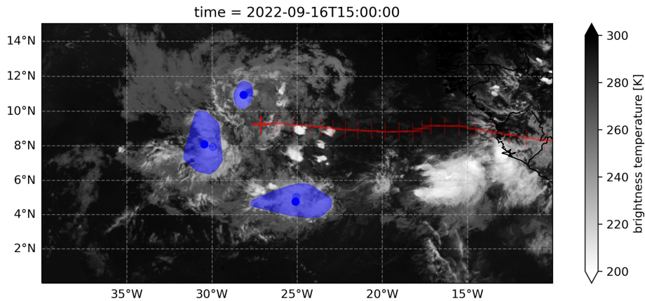
Figure 2. Identified MCSs using MSG data during research flight 7 of the CPEX-CV field campaign. CEs (convex-hull, warm-core 235 K areas) are in blue and IR shaded. Blue dots represent the geographical centroid position. Red crosses are the track of the AEW. Time is in UTC.
