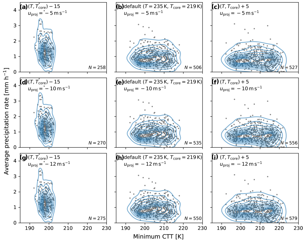
Figure 11. 2-D precipitation rate versus minimum T_b kernel density estimates (KDEs) for simulated MCSs from MPAS sample data interpolated to a latitude–longitude grid. Rows represent results using the same projection speeds for tracking, while columns represent different temperature thresholds for identification. The data are for the period of 8 September 2006 at 12:00 UTC to 13 September 2006 at 18:00 UTC, as in Fig. 5.
