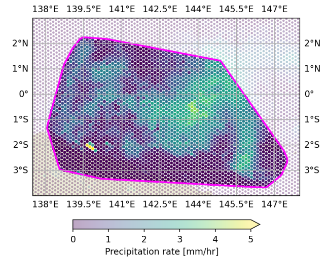
Figure 9. Visualization of the variable assignment of precipitation within a CE selected from Fig. 3b.
