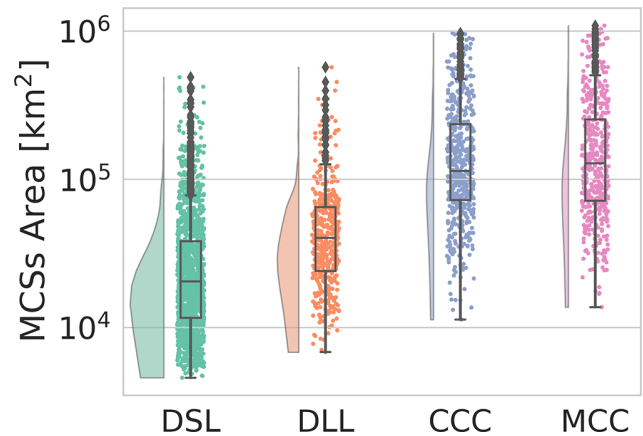
Figure 8. Rain-cloud plots of MCS area (note the log scale) by category for the same period and domain as in Fig. 7.
