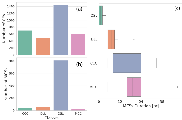
Figure 7. Example statistics for the observed number of CEs (a) and MCSs (b), as well as the duration of MCSs by category (c) during 4 through 30 September 2022, the period of the CPEX-CV field campaign, over a western African domain.
