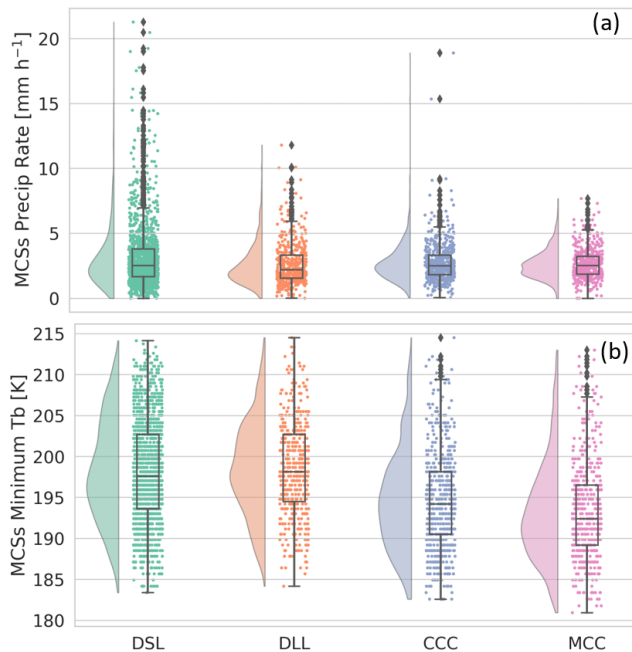
Figure 10. Rain-cloud plots of MCS area-mean rain rates (a) and MCS minimum T_b (b) by category for the same period as in Fig. 7.
