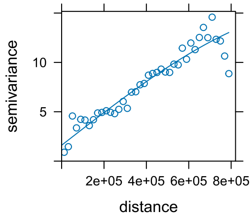
Naive: EDF
