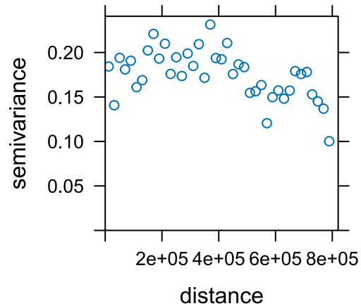
Complete: Baseline
