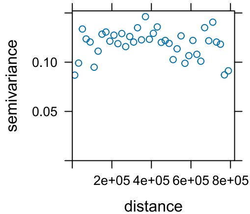
Complete: Coordinates
