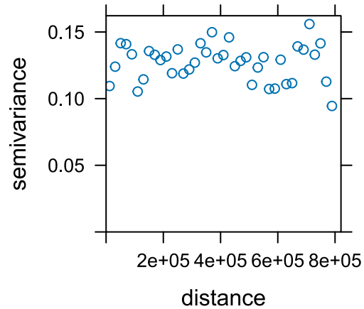
Complete: RFsp
