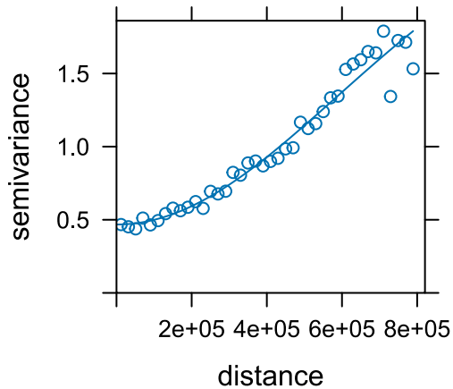
Naive: RFsp
