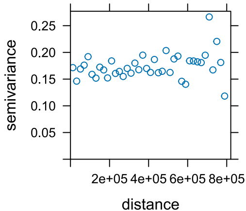
Complete: EDF
