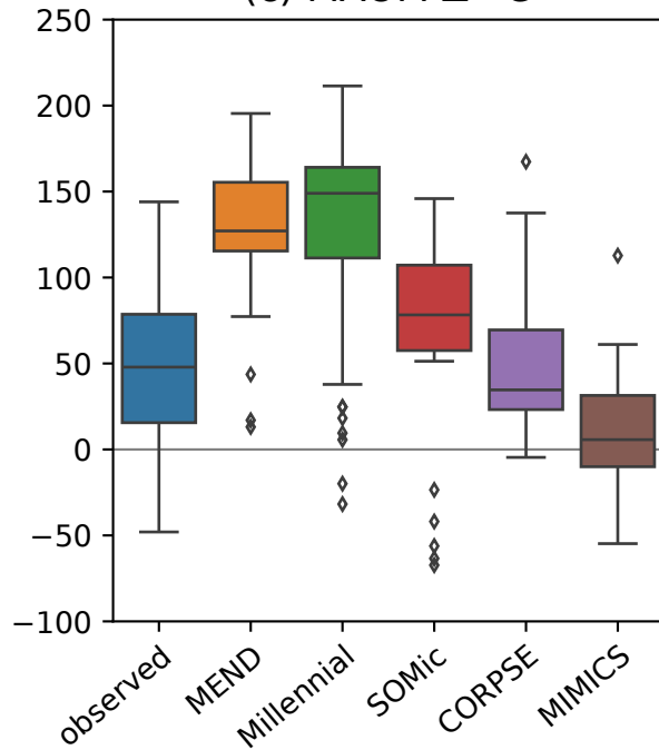
(c) MAOM \Delta^{14}\text{C}
