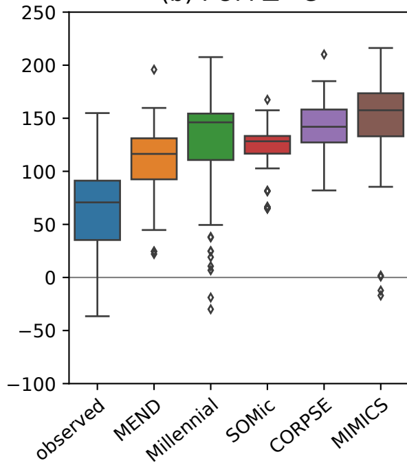
(b) POM \Delta^{14}\text{C}
