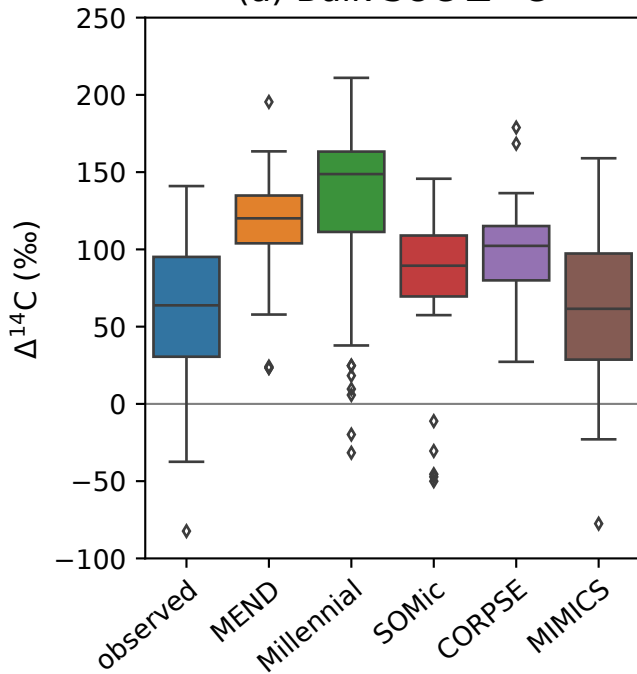
(a) Bulk SOC \Delta^{14}\text{C}
