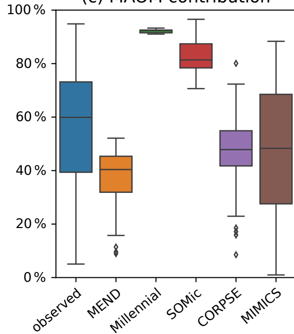
(c) MAOM contribution
