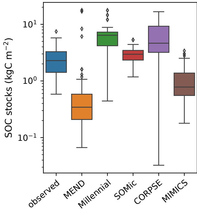
(a) SOC stocks
