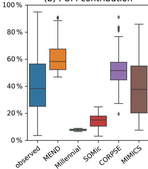
(b) POM contribution
