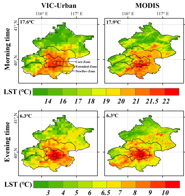
Figure 3. Spatial distribution of the simulated LST compared to the MOD11A2 product, with the average LST shown in the upper left of each panel.
