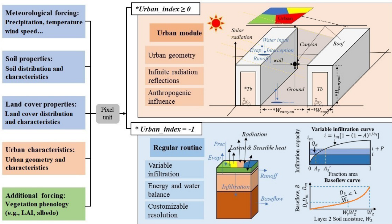
*Urban_index: the number of the urban tile in the target grid ( \geq 0 ), and is equal to -1 if there is no urban tile within the pixel.
