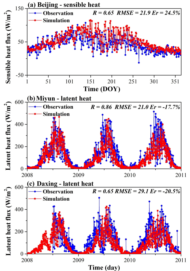
Figure 8. Evaluation of the sensible and latent heat flux simulations: (a) averaged daily sensible heat flux at the Beijing flux tower during 2013–2014, (b) daily latent heat flux at the Miyun flux tower during 2008–2010, and (c) daily latent heat flux at the Daxing flux tower during 2008–2010.
