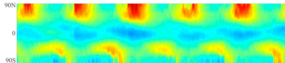
(b) pre-UCX GEOS-Chem adjoint forward component
