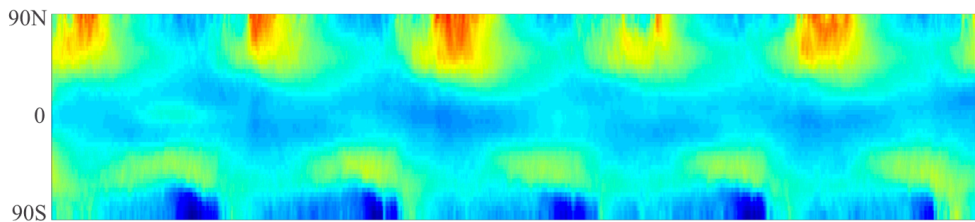
(a) standalone forward GEOS-Chem UCX model
