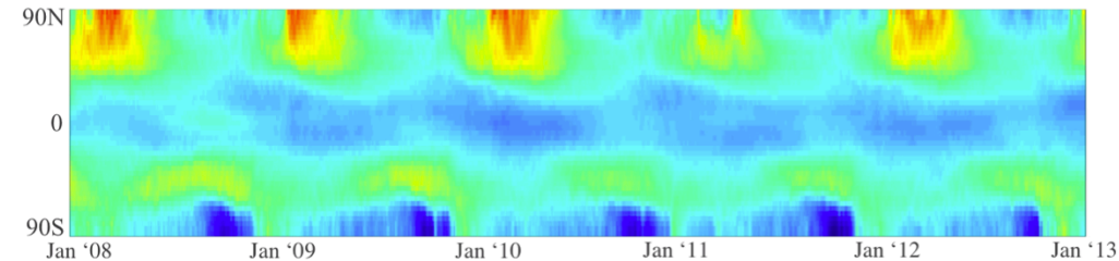
(c) GEOS-Chem UCX adjoint forward component
