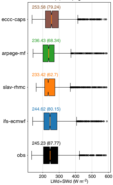
Radiation (e) Utqiagvik
