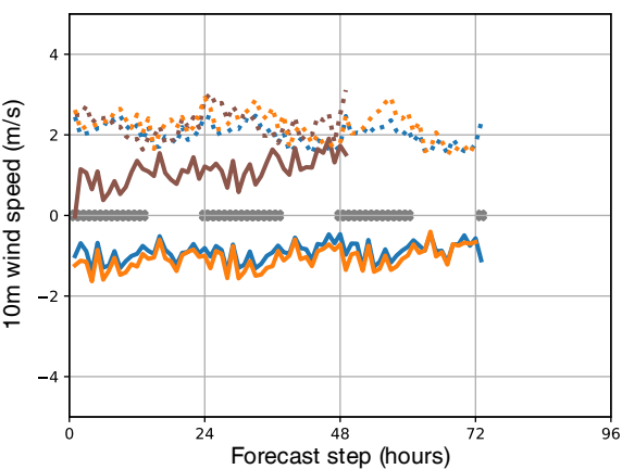
(g) Eureka
