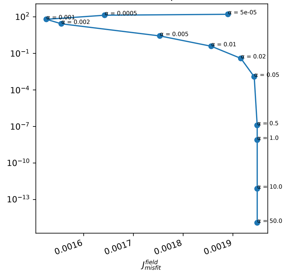
'Gaussian' interpolation
