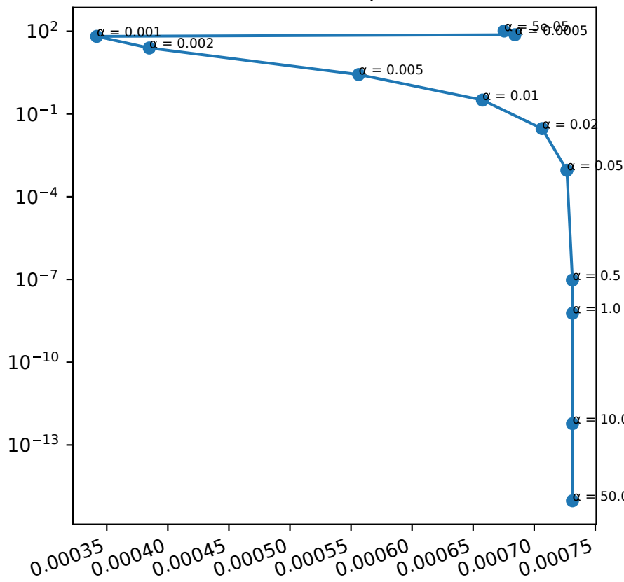
'Clough-tocher' interpolation
