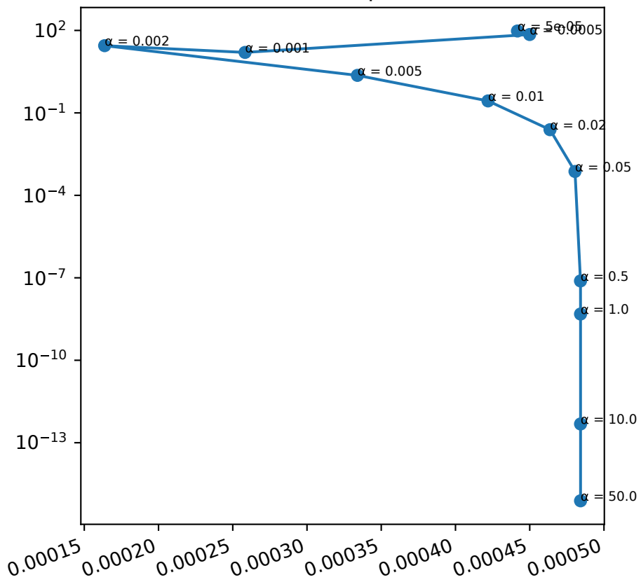
'Gaussian' interpolation
