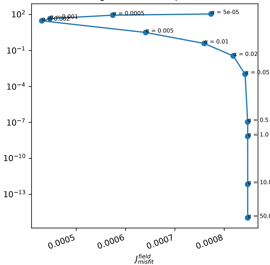
'Clough-tocher' interpolation
