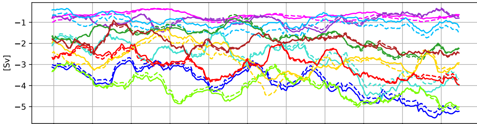
Volume Transport
