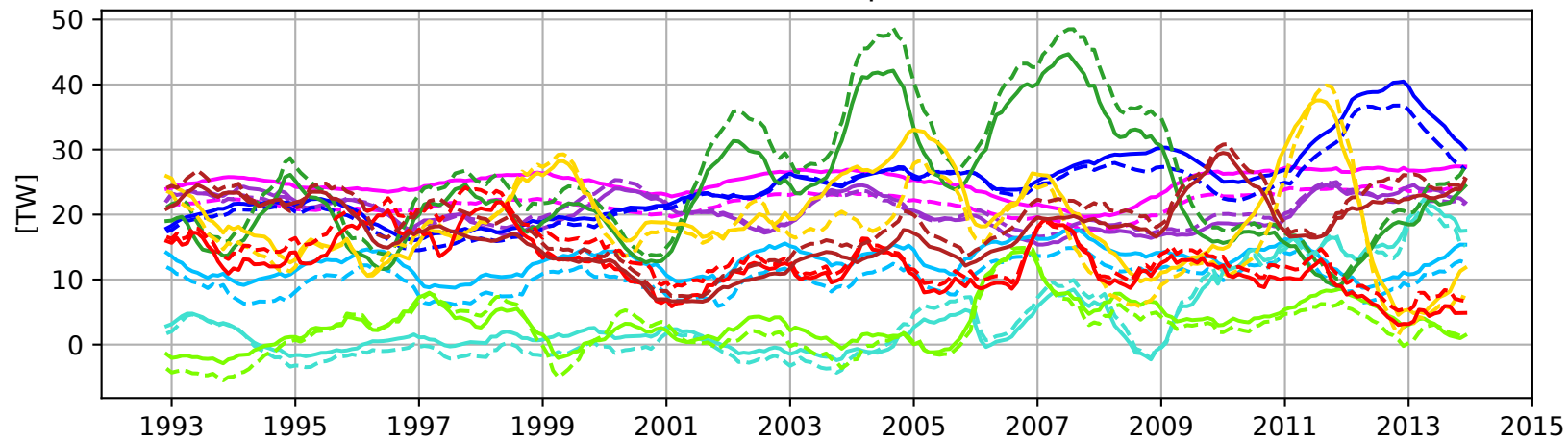
Heat Transport
