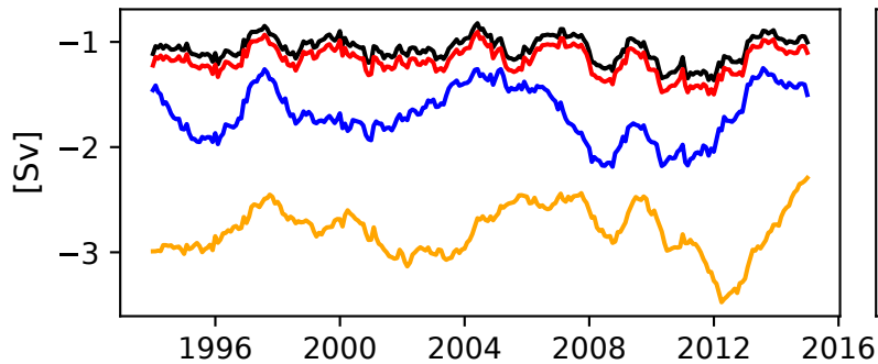
(a) RAPID volume transports
