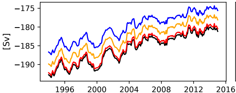
(c) Drake volume transports
