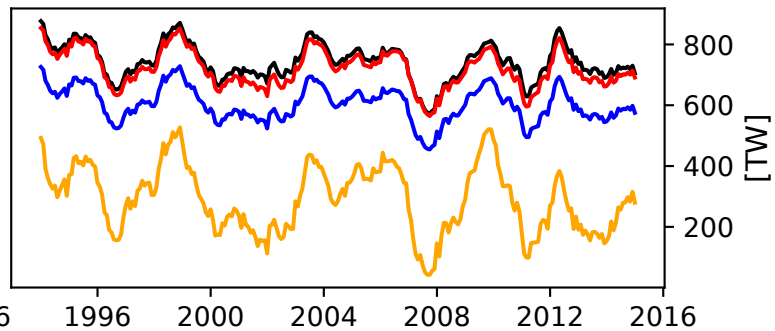
(b) RAPID heat transports
