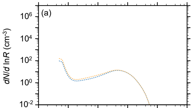
Background conditions
