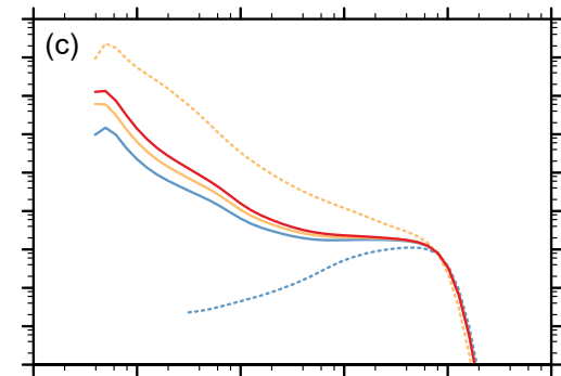
25 Tg(S)/yr injection
