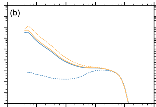
5 Tg(S)/yr injection
