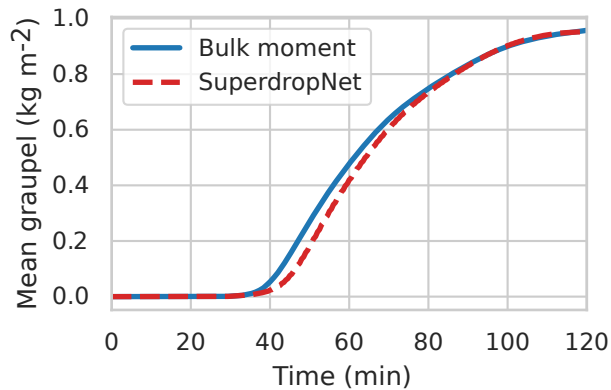
(c) Graupel
