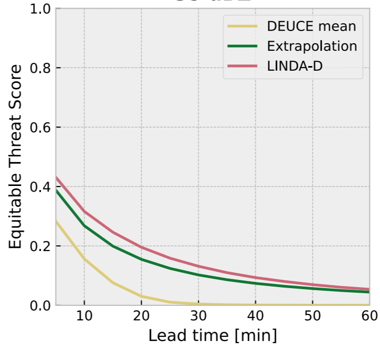
35 dBZ
