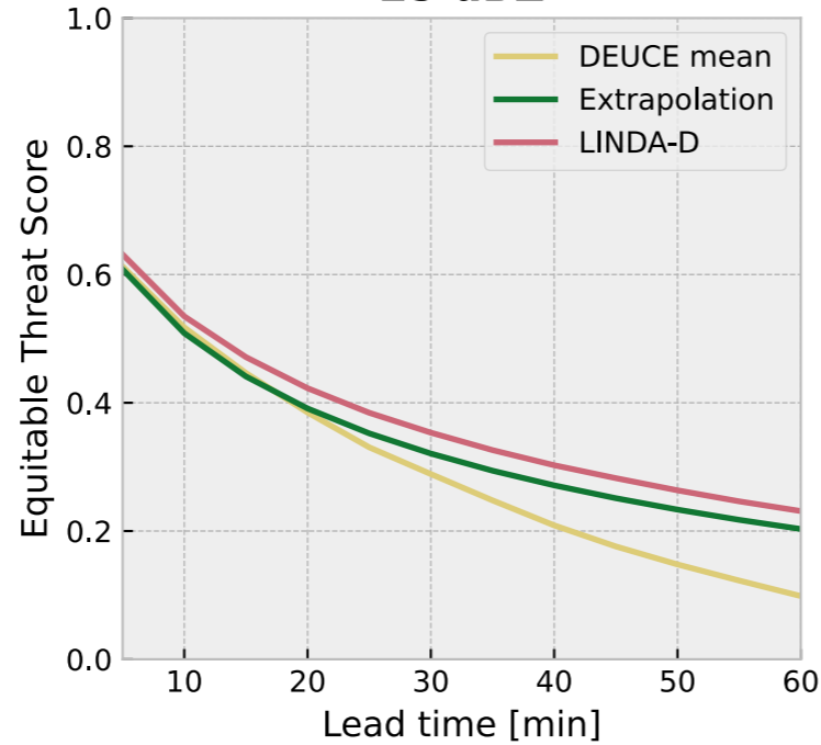
25 dBZ
