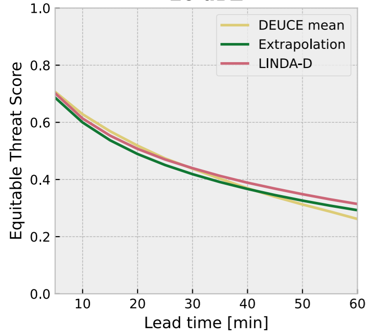
20 dBZ
