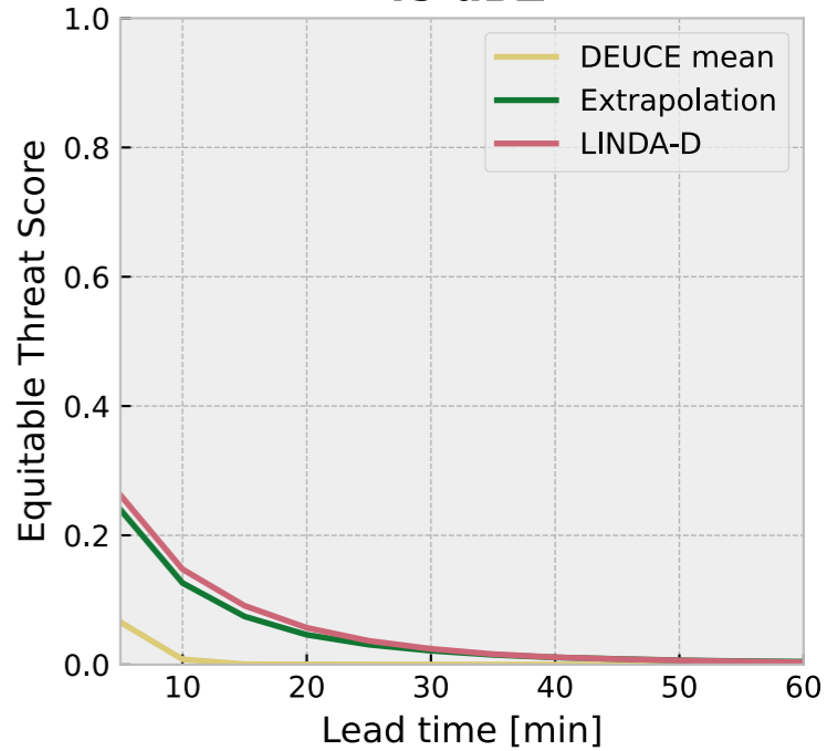
45 dBZ
