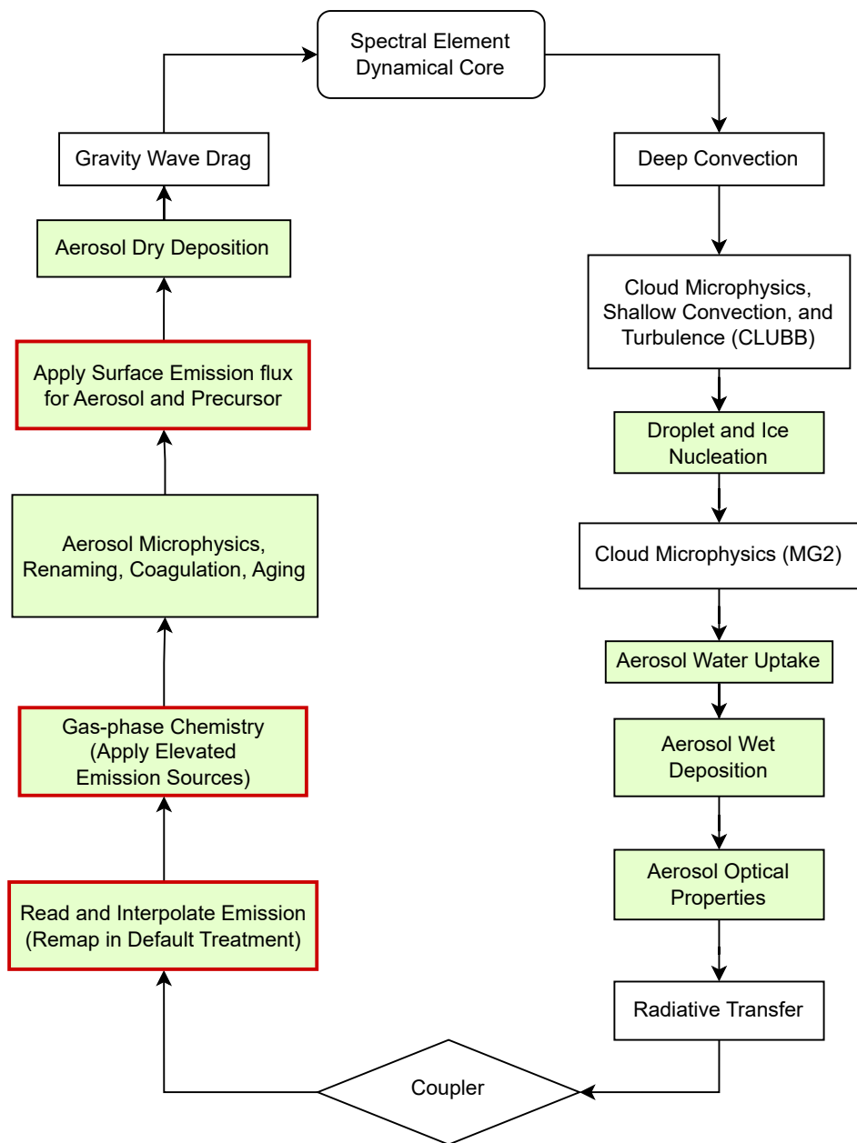
(a) Emission Treatment in EAMv2
