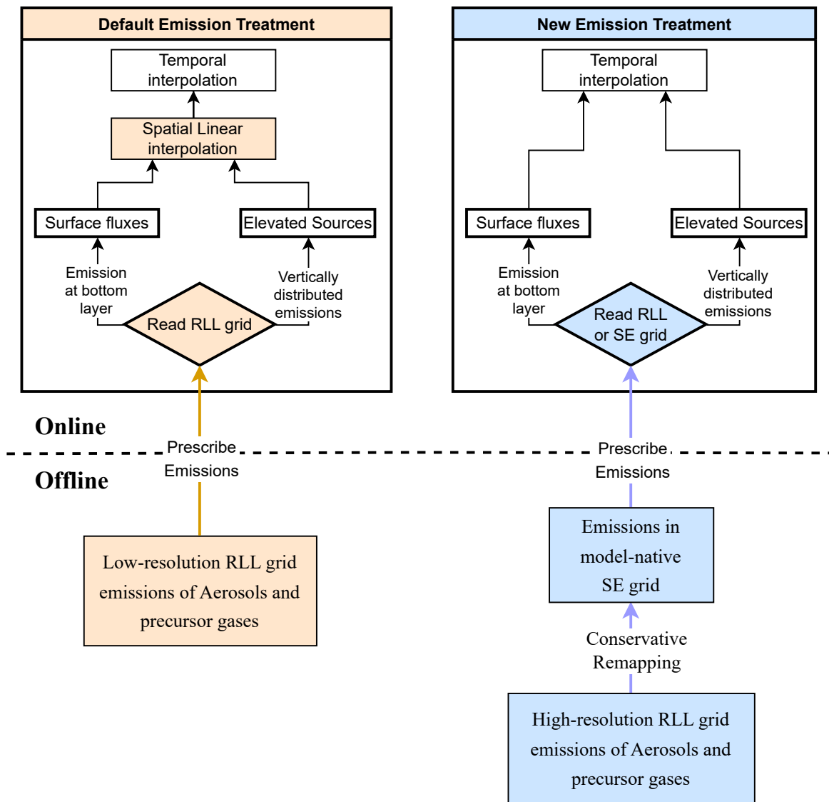
(b) Default vs New Emission Treatment
