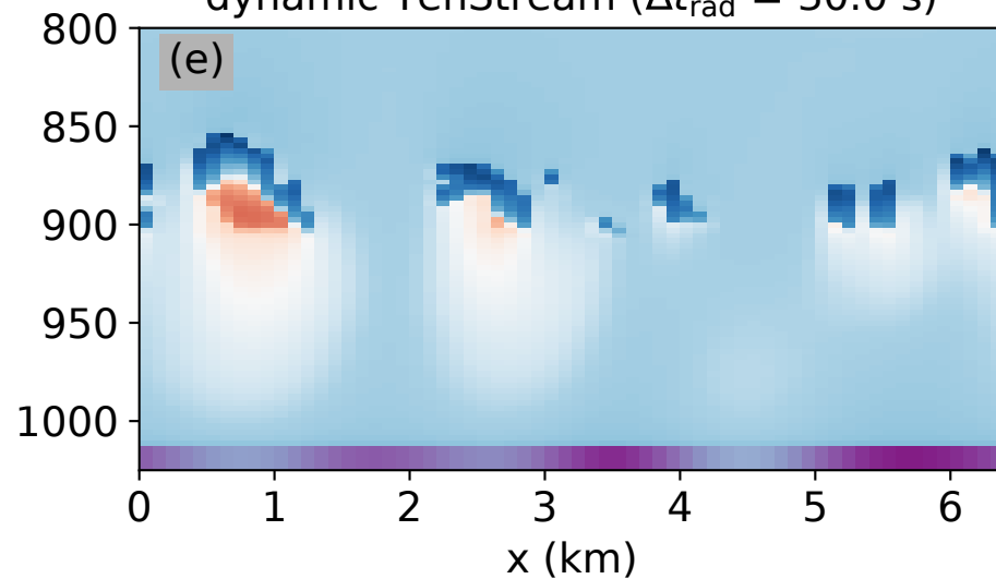
dynamic TenStream ( \Delta t_{\text{rad}} = 30.0 s)
