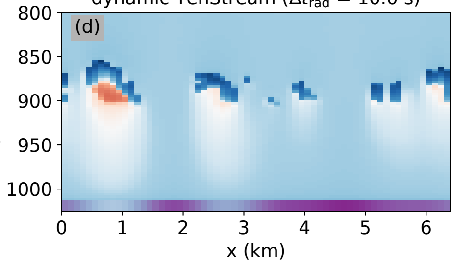
dynamic TenStream ( \Delta t_{\text{rad}} = 10.0 s)
