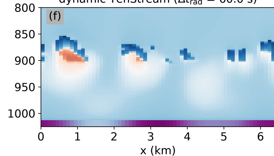
dynamic TenStream ( \Delta t_{\text{rad}} = 60.0 s)
