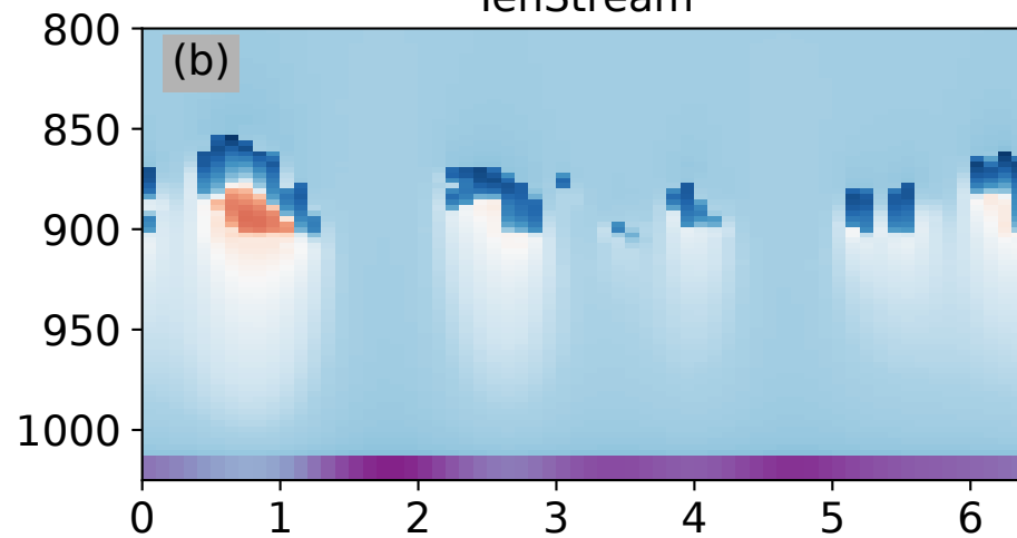
dynamic TenStream ( \Delta t_{\text{rad}} = 30.0 s)
