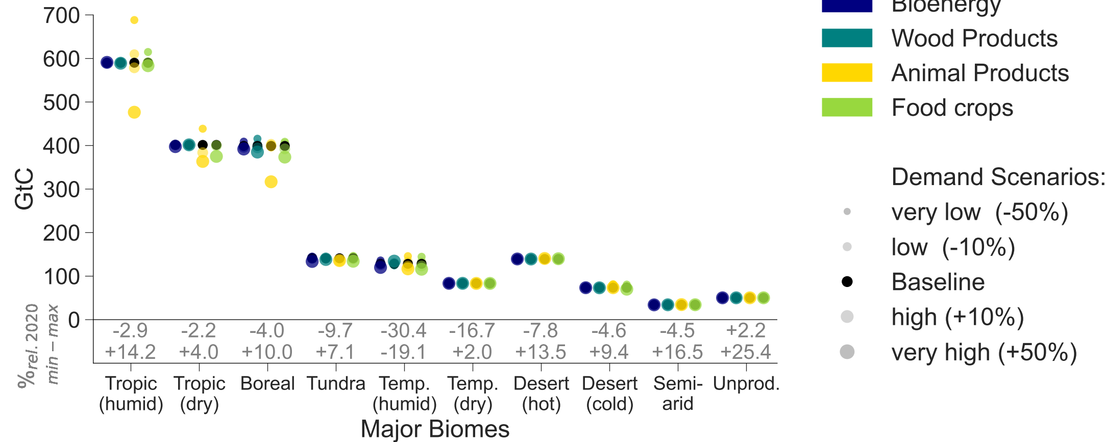
(b) Carbon Stock in 2100
