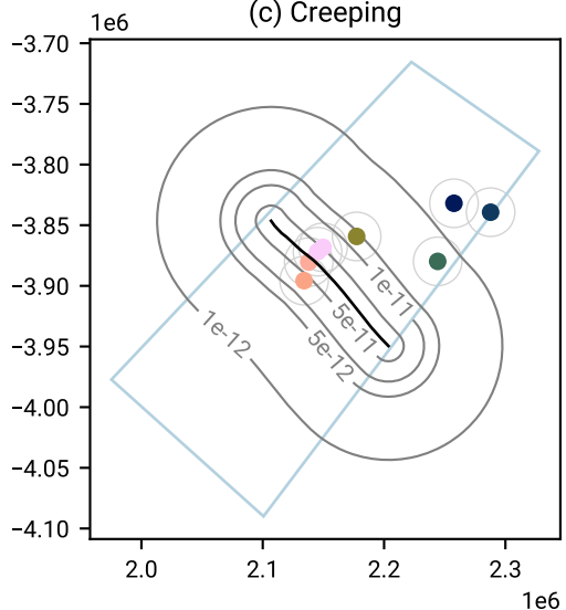
(c) Creeping
