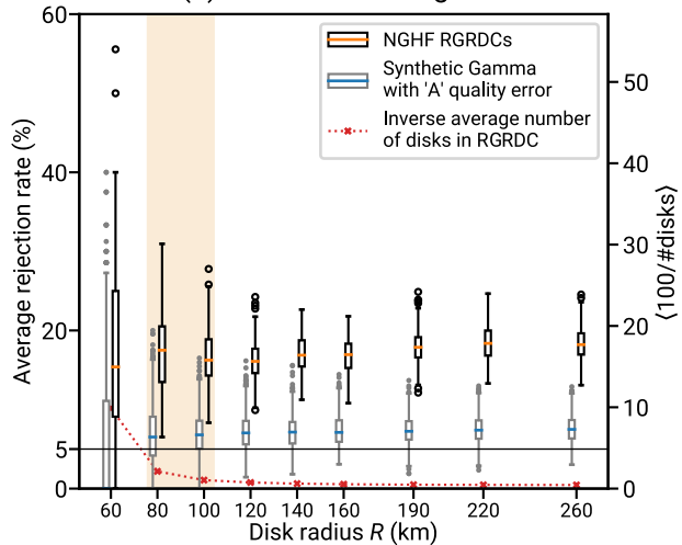
(b) Anderson-Darling test
