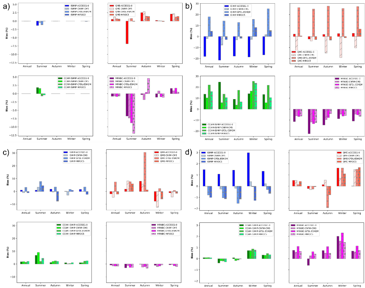
Figure S7: Same as Figure 9, but for the Southern and Southwestern Flatlands (SSWF) NRM region.
