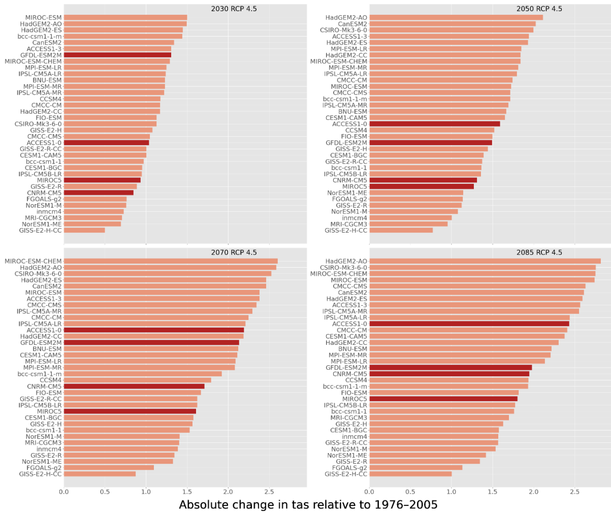
Figure S1: The same as Figure 2 for RCP4.5.
