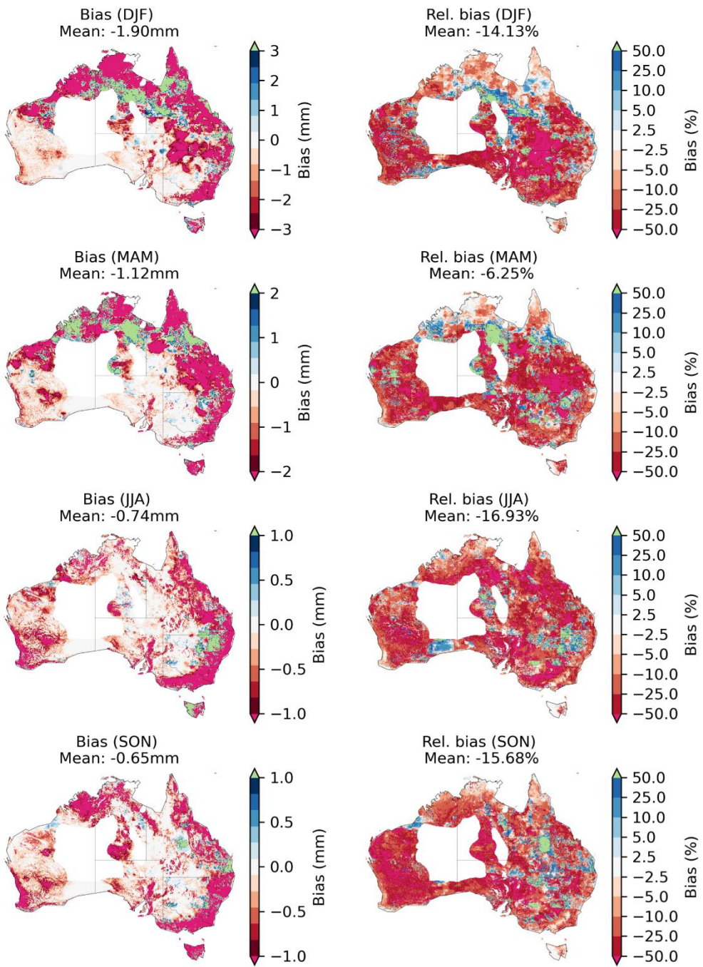
Figure S4: The same as Figure 8(b) but for seasonal values of runoff.
