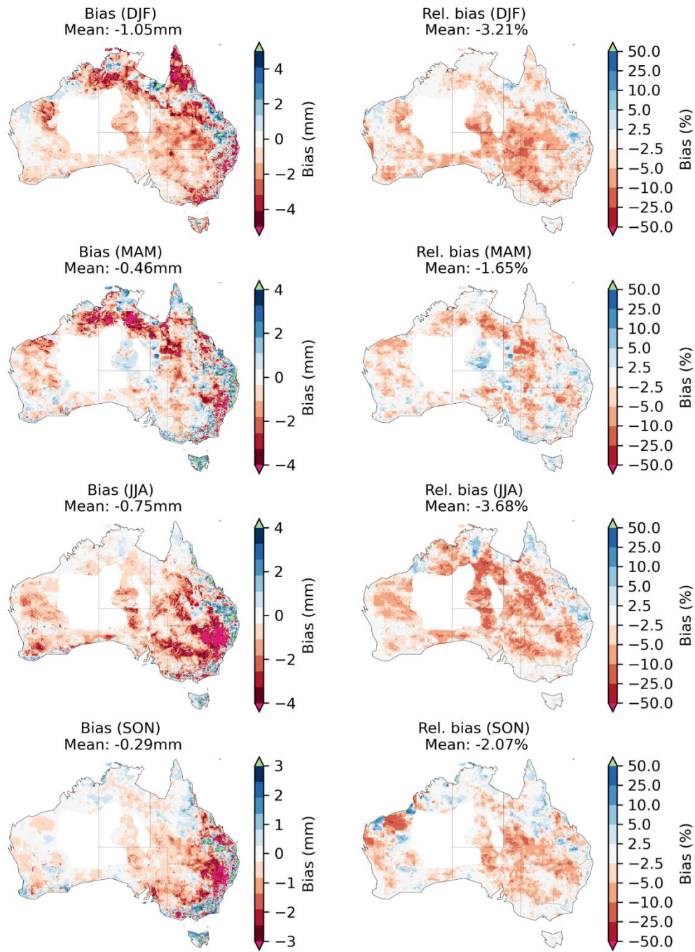
Figure S5: The same as Figure 8(c) but for seasonal values of root-zone soil moisture.
