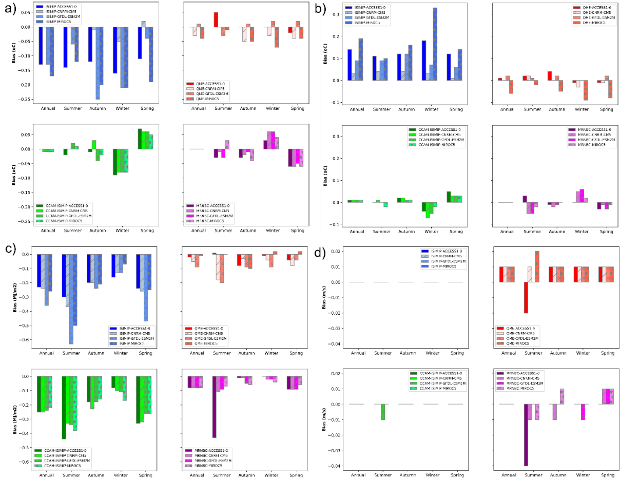
Figure S8: Same as Figure 10, but for the Southern and Southwestern Flatlands (SSWF) NRM region.
