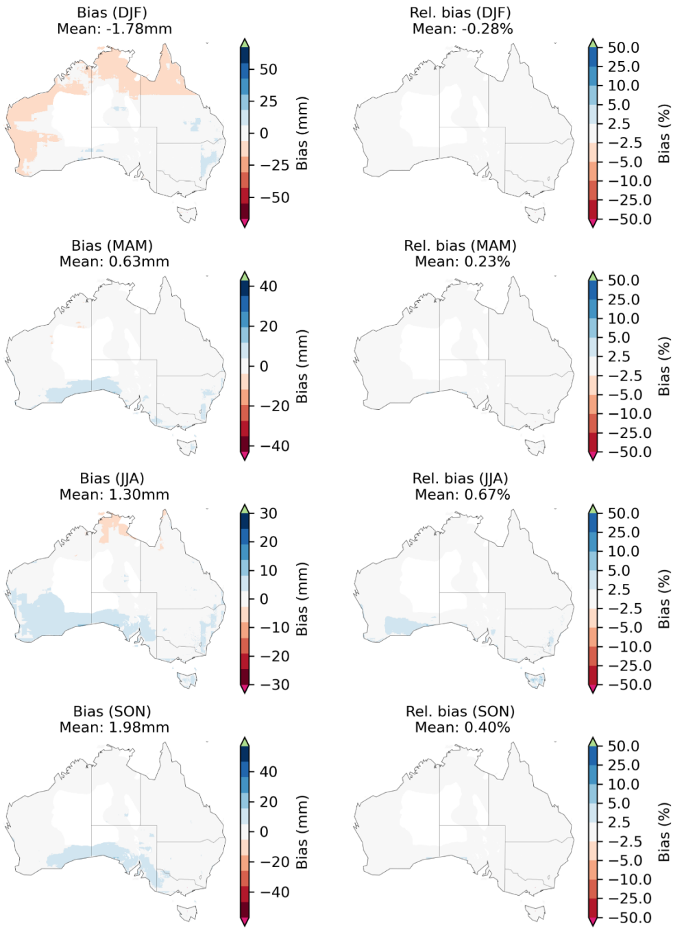
Figure S6: The same as Figure 8(d) but for seasonal values of potential evapotranspiration.
