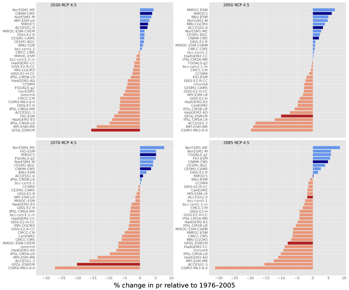
Figure S2: The same as Figure 3 for RCP4.5.
