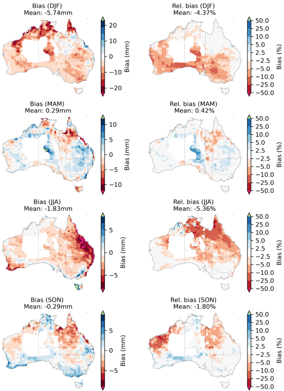
Figure S3: The same as Figure 8(a) but for seasonal biases of precipitation.
