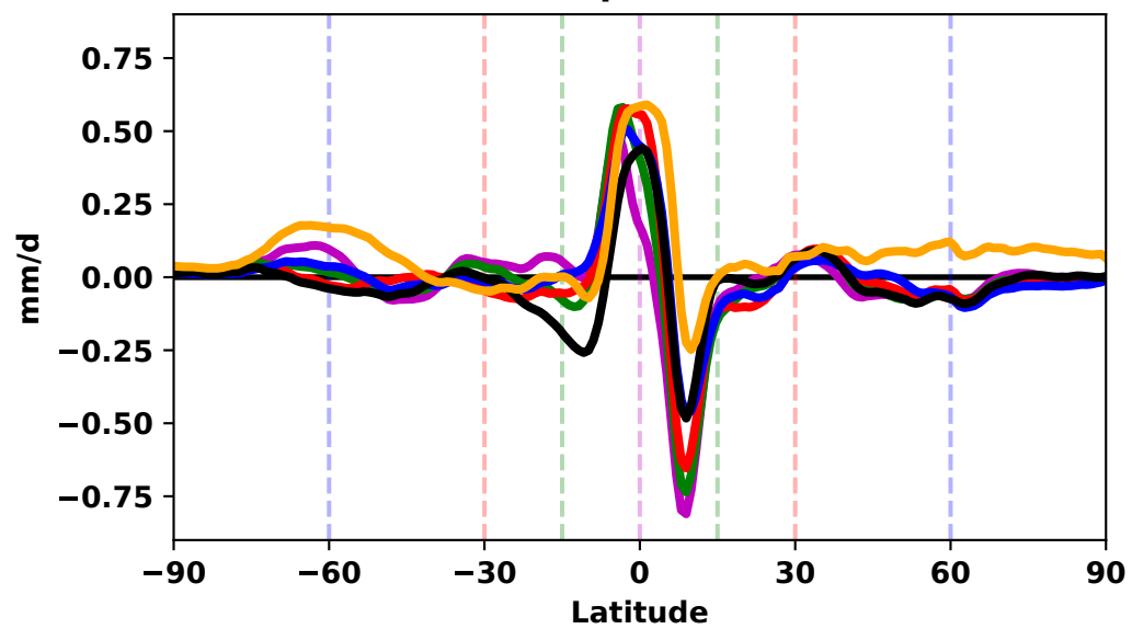
(f) CESM2 \Delta Precipitation (2050-2069)
