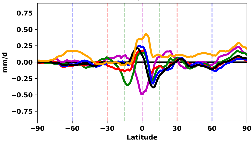
(e) UKESM1 \Delta Precipitation (2050-2069)
