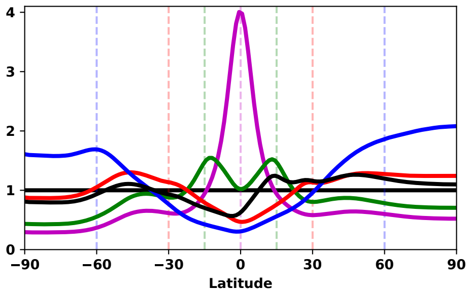
(c) UKESM1 \Delta Ts (2050-2069)
