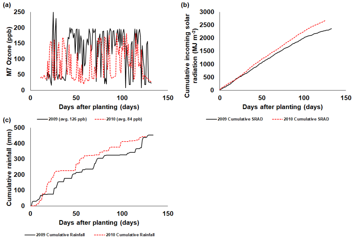
Figure S4. (a) Daily mean 7-hour O 3 concentrations of the highest O 3 treatment, (b) cumulative incoming solar radiation, and (c) cumulative rainfall for the 2009 (solid line) and 2010 (dashed line) growing seasons of the SoyFACE experiment conducted at Champaign, IL, USA.
