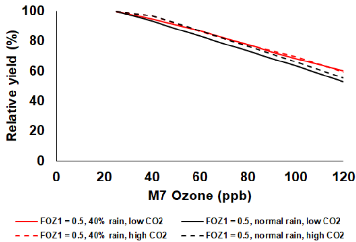
Figure S5: Sensitivity analysis using the CERES-Maize model to simulate relative yield due to elevated O 3 stress for an example of FOZ 1 set at 0.5 under the 40% reduced rainfall and 350 ppm CO 2 (solid red line), normal rainfall and 350 ppm CO 2 (solid black line), 40% less rainfall and 550 ppm CO 2 (dashed red line), and normal rainfall and 550 CO 2 (dashed black line) scenarios. The Champaign, Illinois, USA 2018 FACE weather, soil, and dominant management conditions were used for the reference location. FOZ 1 was tested independently, i.e., SFOZ 1 was set to zero. The 50% reduced rainfall shown in Fig. 4c had low simulated water deficit stress which obscured the O 3 -water stress dynamics. Reducing the rainfall to 40% increased simulated water deficit stress to allow for a better representation of the O 3 -water stress dynamics.
