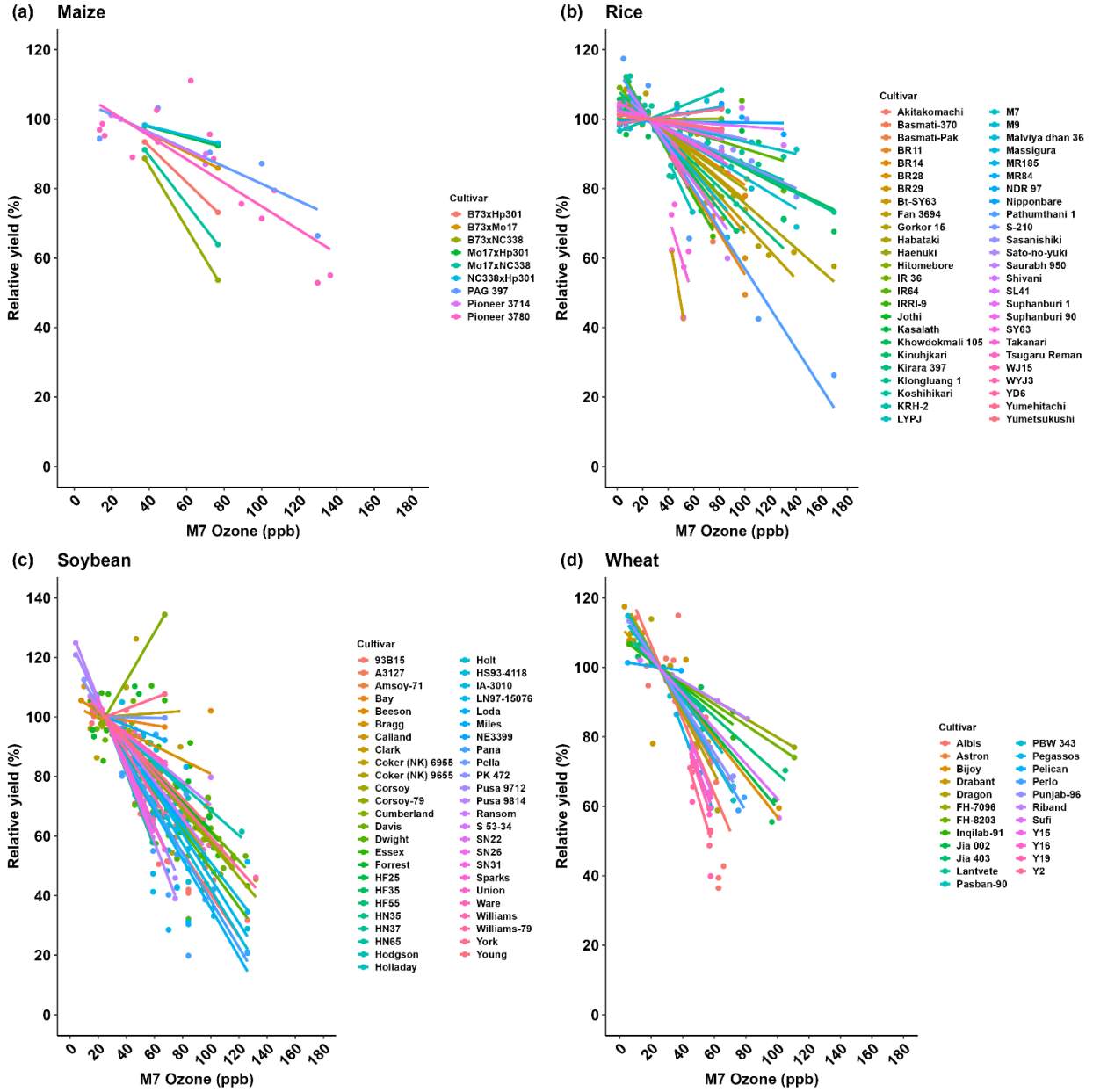
Figure S2: The cultivar O 3 exposure-yield response for increasing M7 O 3 concentrations. The data consists of the relative yields (scaled to 25 ppb M7 O 3 ) of the cultivars examined in the Mills et al. (2018) literature review combined with the maize and soybean cultivars used in this study for a total of (a) 9 maize cultivars, (b) 50 rice cultivars, (c) 49 soybean cultivars, and (d) 23 wheat cultivars (colored symbols). The colored lines show the linear regression of the exposure-yield response for each cultivar. The slope and y-intercept of the linear fit for each cultivar are shown in Table S10.
