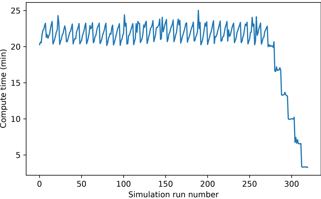
Computing time per eEMEP run on Nebula
