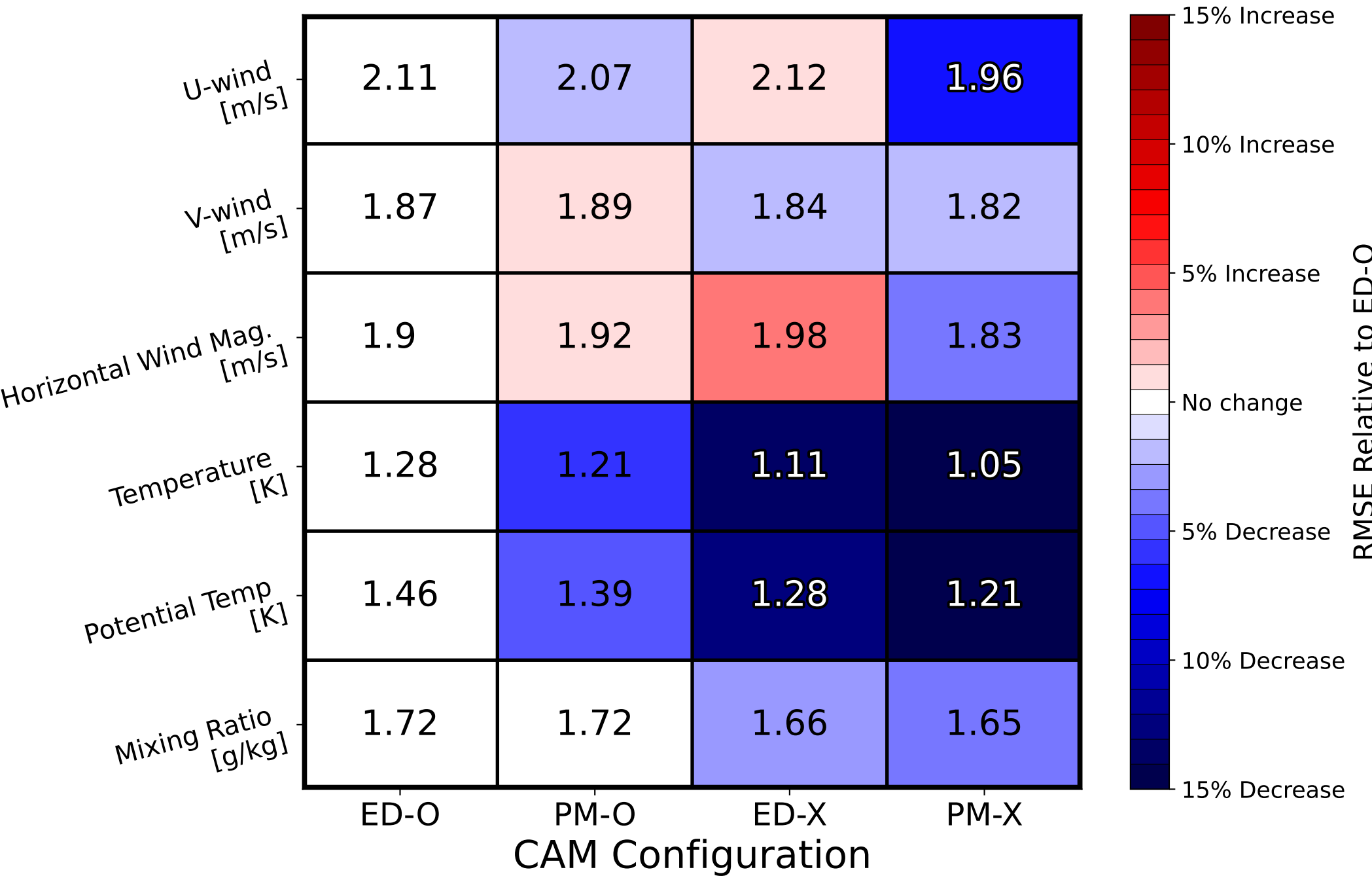
CAM RMSEs Between 200 m and 2000 m Altitude
