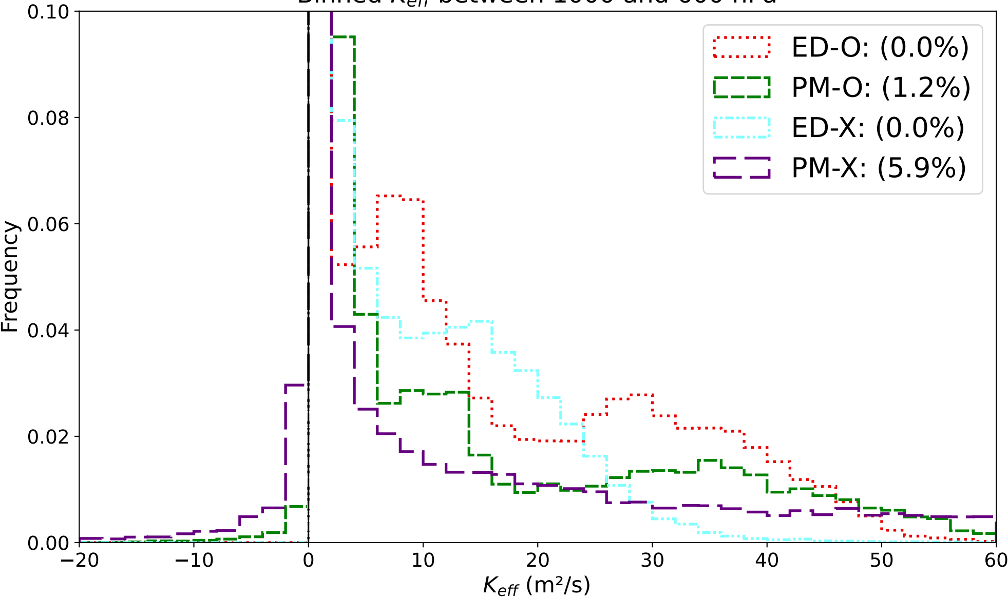
Binned K_{eff} between 1000 and 600 hPa
