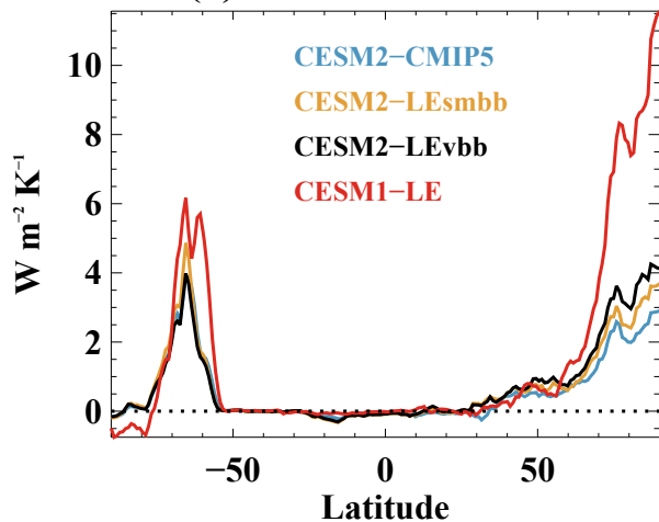
(a) 2000–2020 AlbFB
