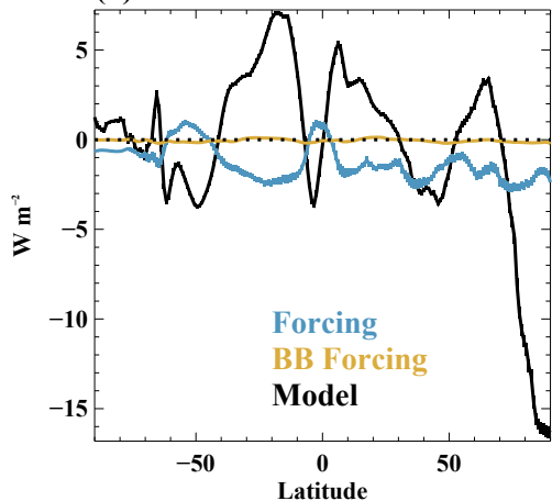
(f) Forcing Attribution \Delta FSNT
