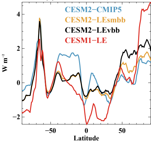
(c) Attribution 2000–2020 \Delta FSNT
