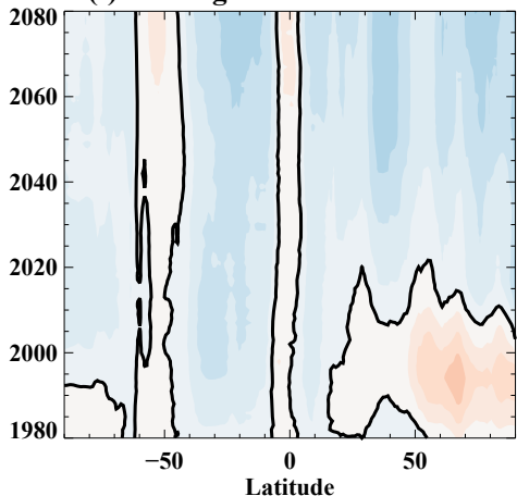
(f) Forcing Attribution \Delta FSNT
