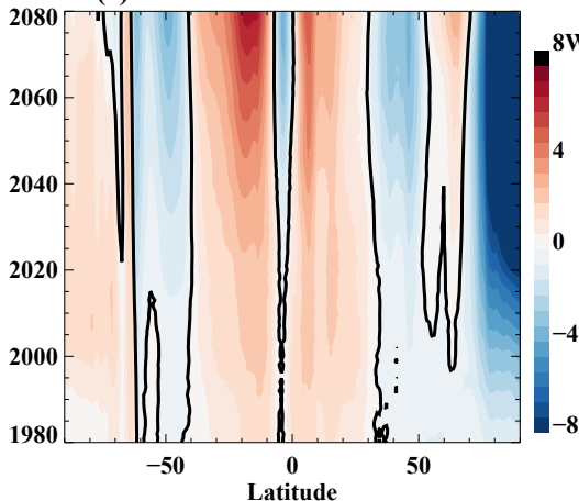
(e) Model Attribution \Delta FSNT
