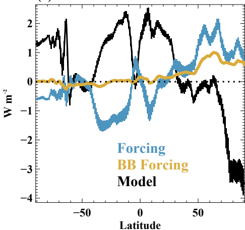
(e) Model Attribution \Delta FSNT
