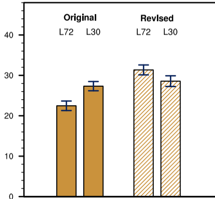
(b) Global burden (Tg)
