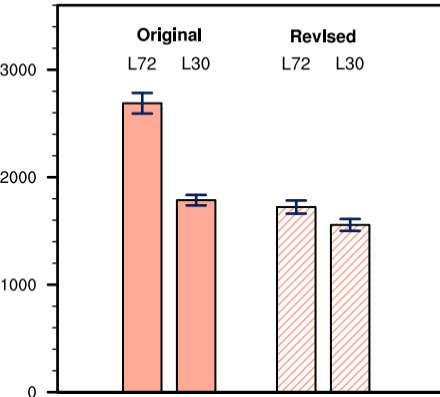
(a) Dry removal in source regions (Tg/yr)
