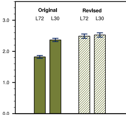
(c) Global mean lifetime (day)
