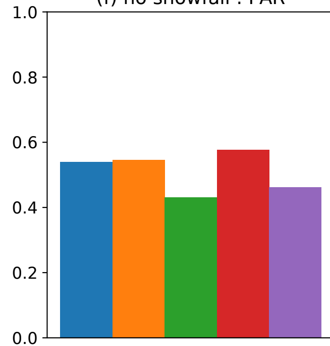
(f) no snowfall : FAR
