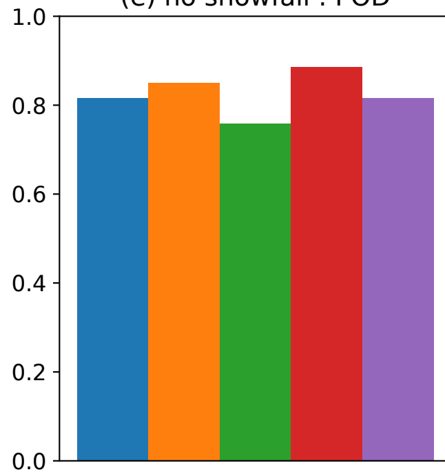
(e) no snowfall : POD
