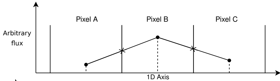
Linear centred scheme
