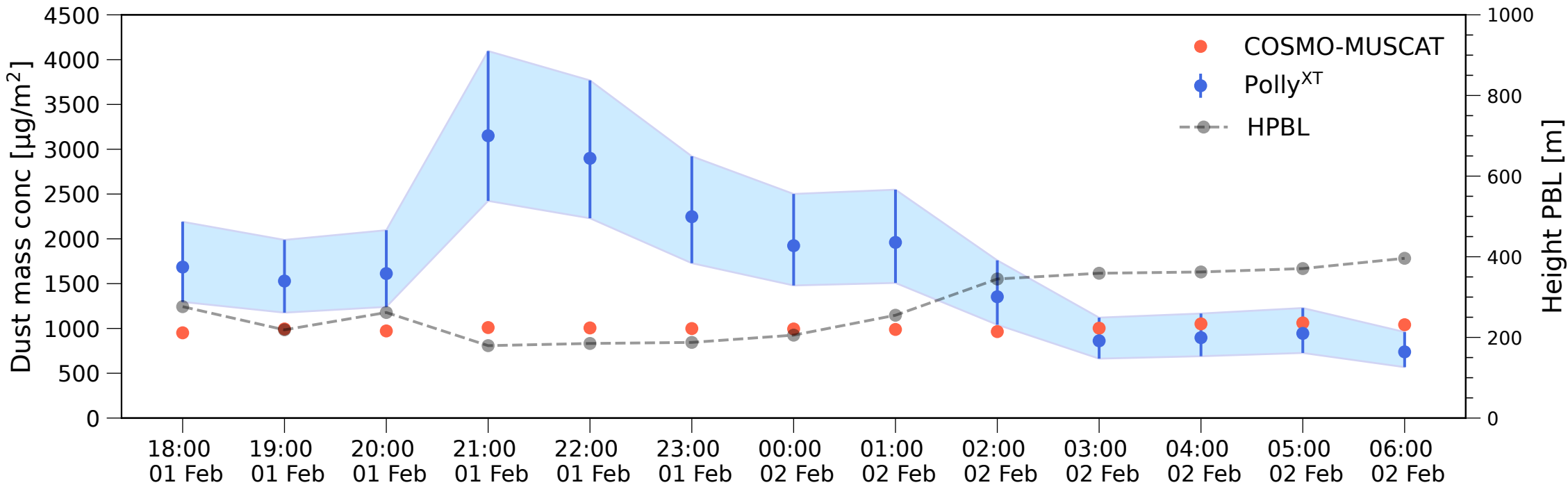
Column dust mass concentrations at Mindelo above PBL
