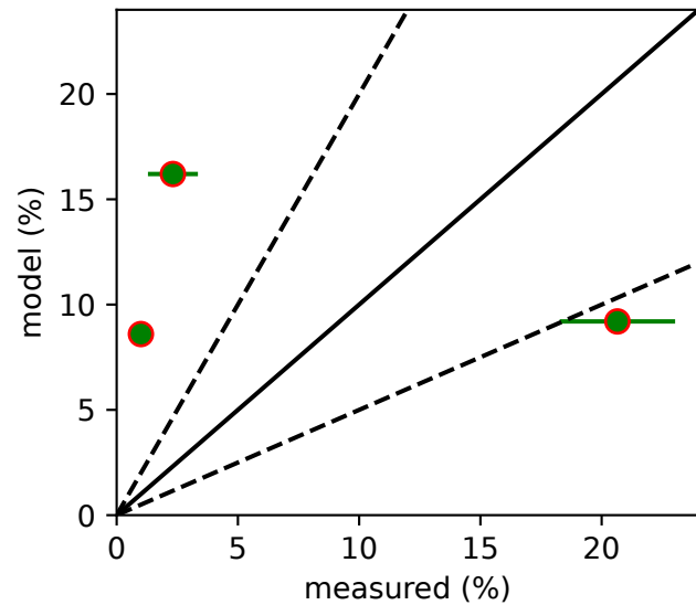
Quartz
