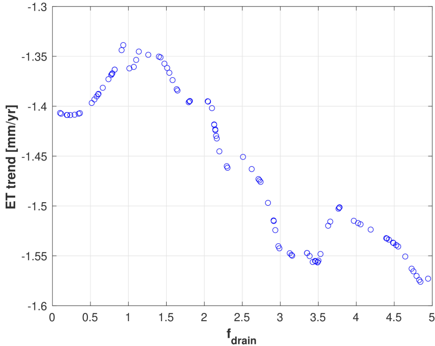
(b) Sensitivity of ET to f_{drain}
