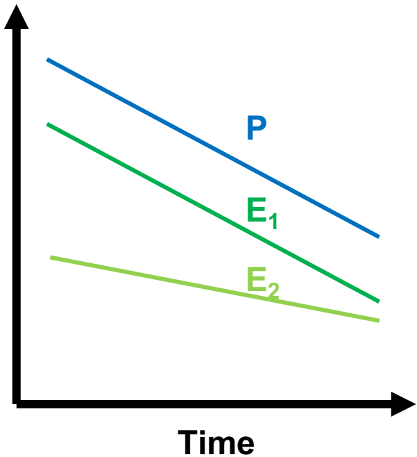
(a) Decreasing trend in runoff
