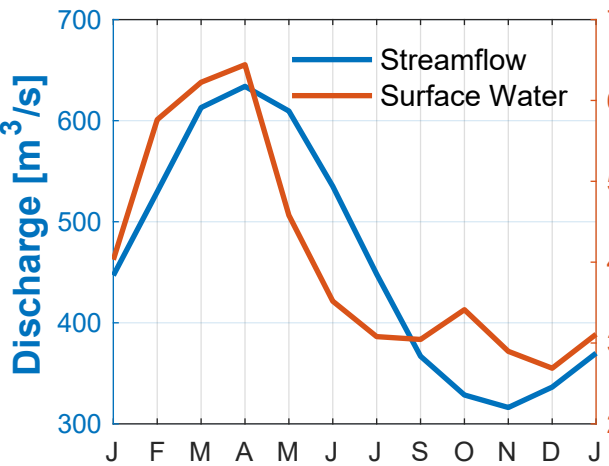
Subbasin #1
