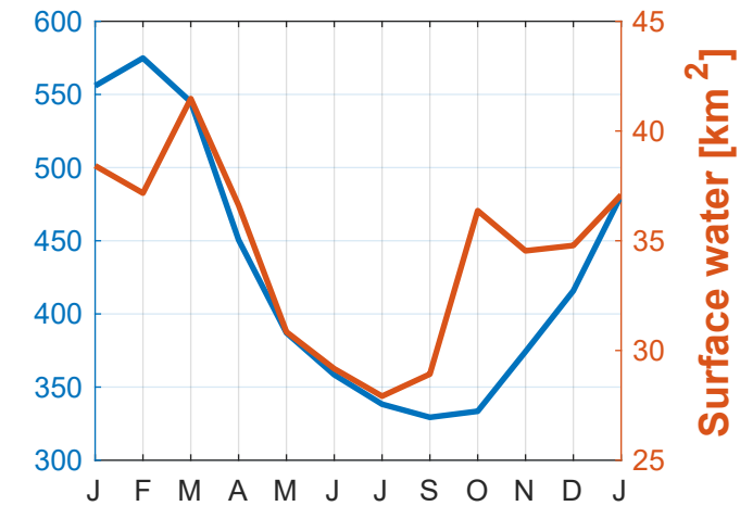
Subbasin #3
