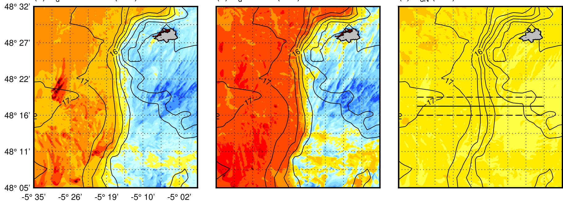
(a) C_d COARE3.0 ( 10^{-3} )
