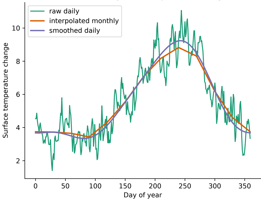
Mean annual cycle of temperature change
