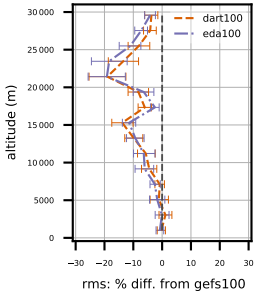
(b) refractivity (N-units) at 2.0 d
