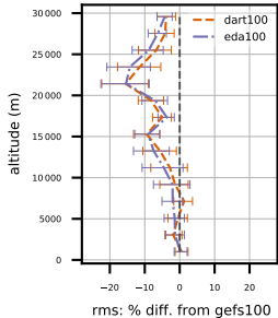
(c) refractivity (N-units) at 3.0 d
