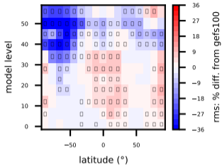
(b) dart100 T (C)
