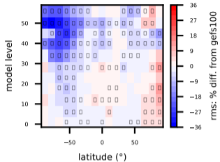
(c) eda100 T (C)
