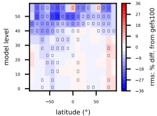
(f) eda100 U (m/s)
