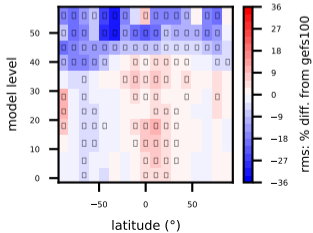
(e) dart100 U (m/s)
