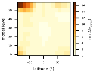
(a) gefs100 T (C)
