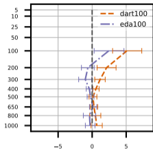
(a) U (m/s) at 1.0 d
