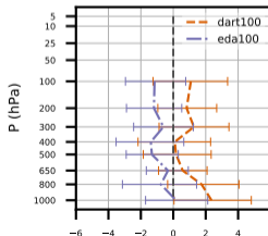
(f) V (m/s) at 3.0 d
