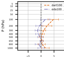
(b) U (m/s) at 2.0 d
