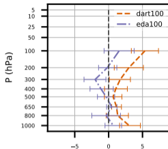
(c) U (m/s) at 3.0 d
