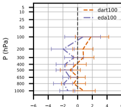
(e) V (m/s) at 2.0 d
