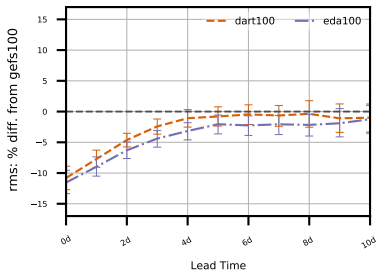
(c) U (m/s)
