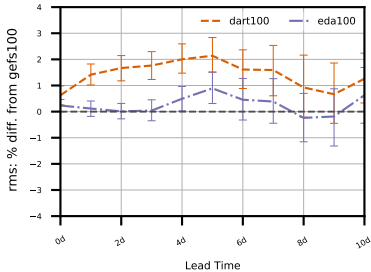
(b) Qv (g/kg)
