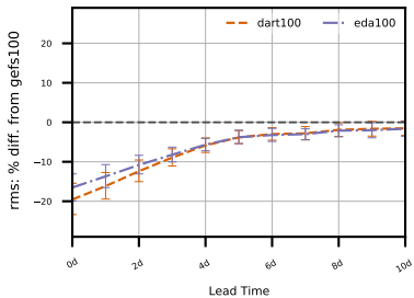
(a) T (C)
