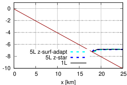
(c) channel Free surface at t=21600.0 s
