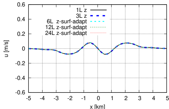
impulsiveWave x-velocity at t=3.0 s
