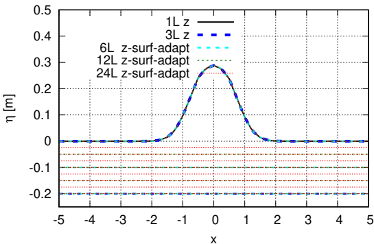
impulsiveWave Free surface at t=0.3 s
