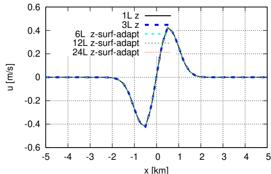
impulsiveWave x-velocity at t=0.3 s
