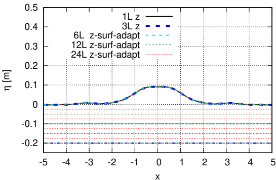
impulsiveWave Free surface at t=3.0 s
