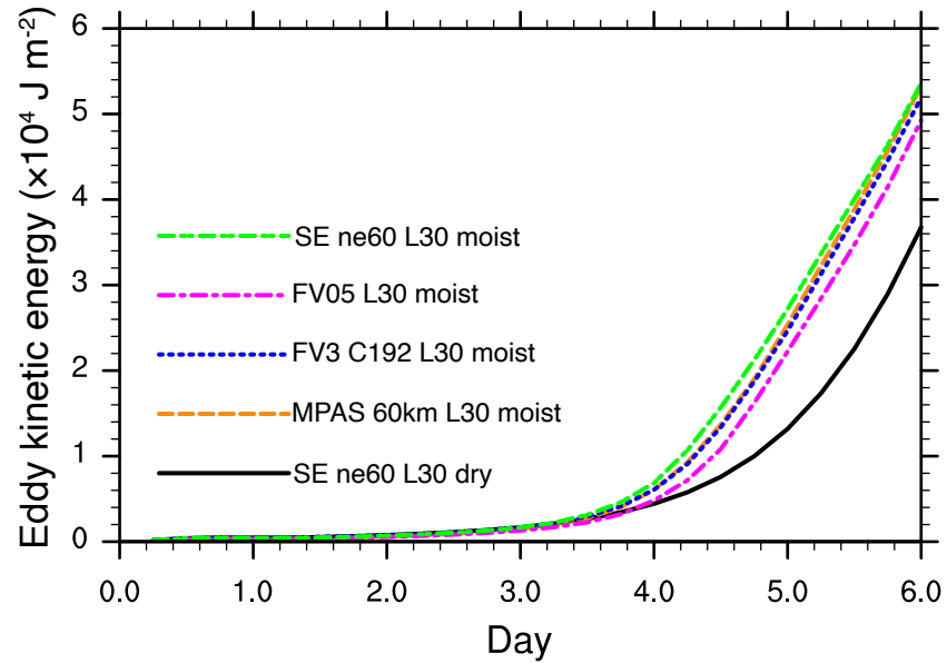
Integrated EKE vs. time
